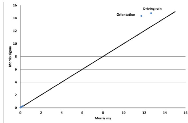
Fig. 8. Morris analysis for average moisture content in the innermost layer of the brick wall
