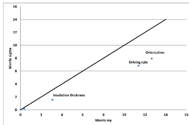
Fig. 9. Morris analysis for average moisture content in the outermost layer of the brick wall
