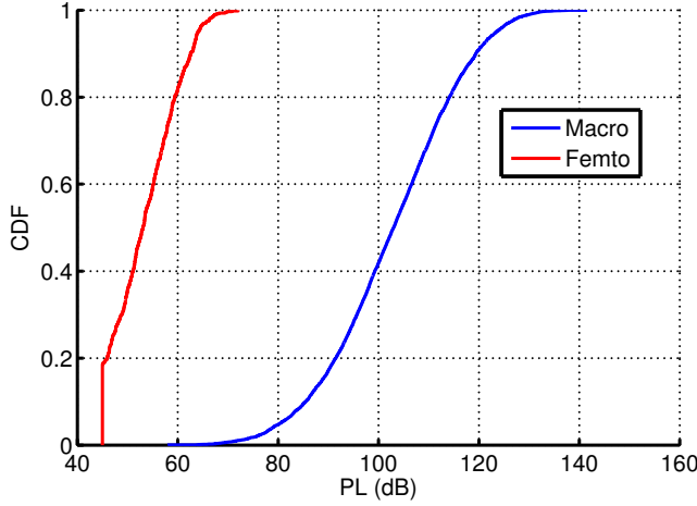
Fig. 4.2: Comparing the path loss distribution to the serving cell in Macro and Femto deployments. The macrocell case was generated assuming the 3GPP Macro-1 scenario corresponding to an inter-site distance of 500 m [63].
