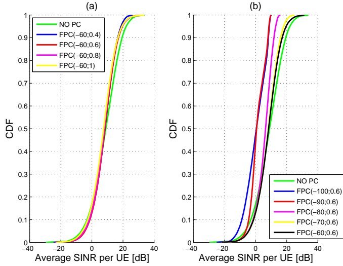
Fig. 4.5: CDFs of uplink SINR (a) for fixed P_0 = -60\text{dBm} and (b) for fixed \alpha = 0.6 compared to no power control under universal frequency reuse. One can observe that P_0 is the dominating factor affecting the average SINR.
