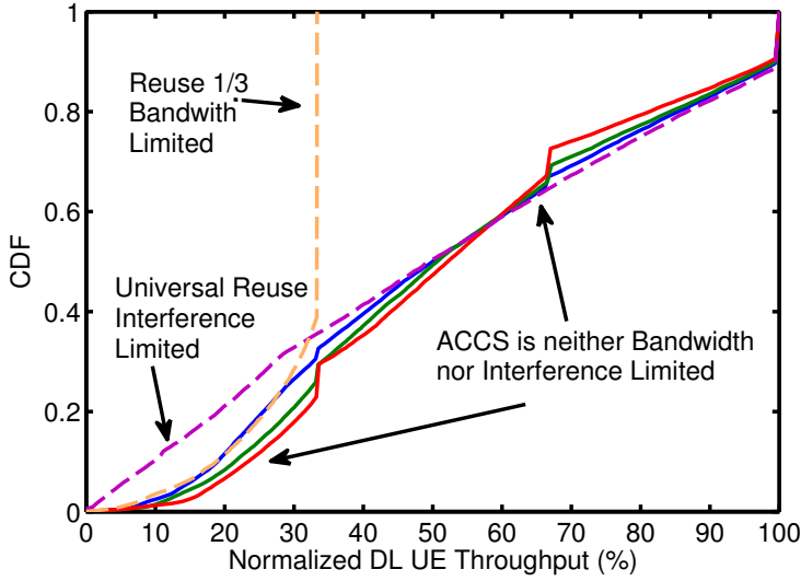
Fig. 3.5: ACCS retains the benefits of both sparse and tight frequency reuse patterns (dashed lines). The three solid lines depict the overall effect of varying the thresholds. By adjusting the CIR targets one can improve the outage performance by shifting the lower tail to the right at the expense of slightly lower average and peak performance.
