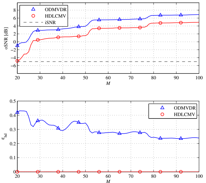
Fig. 12. Performance of the filters as a function of M when the harmonics has decreasing amplitudes and the noise is a sum of sinusoidal noise and white Gaussian noise.
