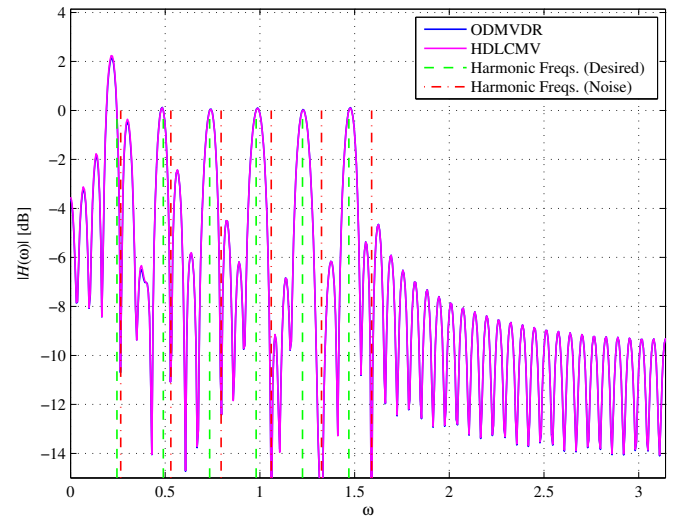
Fig. 4. Magnitude responses of the ODMVDR and HDLCMV filters of order M = 100 designed for a periodic signal corrupted by sinusoidal noise and white Gaussian noise.
