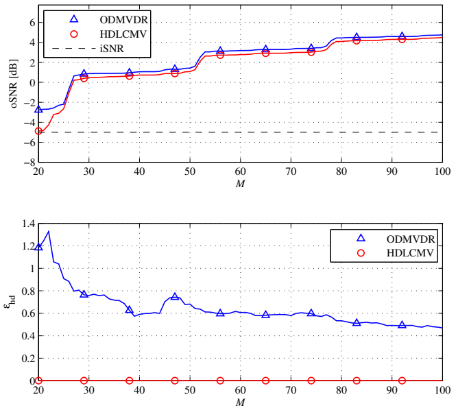
Fig. 11. Performance of the filters as a function of M when the harmonics has unit amplitudes and the noise is a sum of sinusoidal noise and white Gaussian noise.
