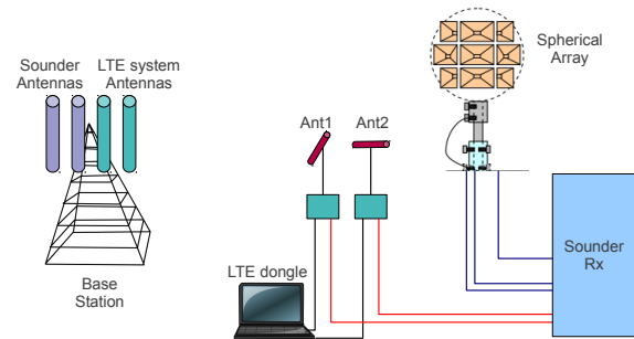
Fig. 1. Schematic of parallel sounding and device performance evaluation in a live LTE system.
