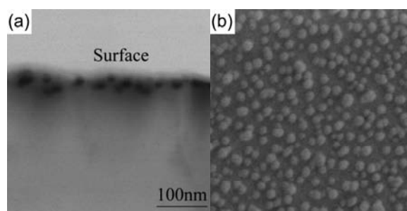
Fig. 9. (a) Scanning TEM image (in cross-section) and (b) SEM image (frame size is 600 \times 600 nm) of PET implanted by 40 keV tungsten ions with fluence of 1 \times 10^{17} \text{cm}^{-2} . Reprinted from [96] with permission from Elsevier.
