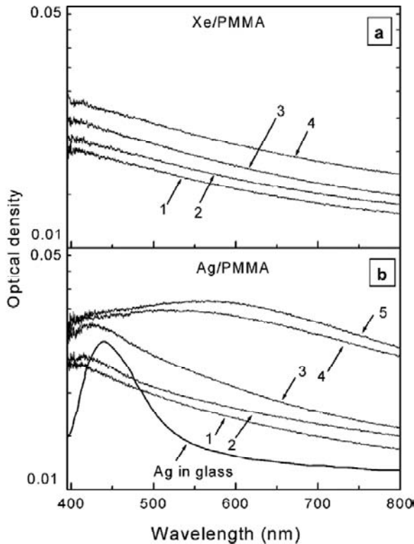
Fig. 26. Optical absorption spectra of PMMA implanted by (a) 30 keV \text{Xe}^+ and (b) \text{Ag}^+ ions with fluences of (1) 3 \times 10^{15} , (2) 6 \times 10^{15} , (3) 2.5 \times 10^{16} , (4) 5 \times 10^{16} , and (5) 7.5 \times 10^{16} \text{ cm}^{-2} . Spectra of unimplanted PMMA and silica glass with Ag NPs formed by implantation are presented for comparison. According to [169].
