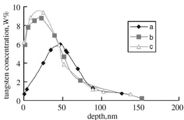
Fig. 8. Depth profiles of 40 keV tungsten implanted into PET with fluencies of (a) 5 \times 10^{16} , (b) 1 \times 10^{17} and (c) 2 \times 10^{17} \text{cm}^{-2} . Reprinted from [96] with permission from Elsevier.
