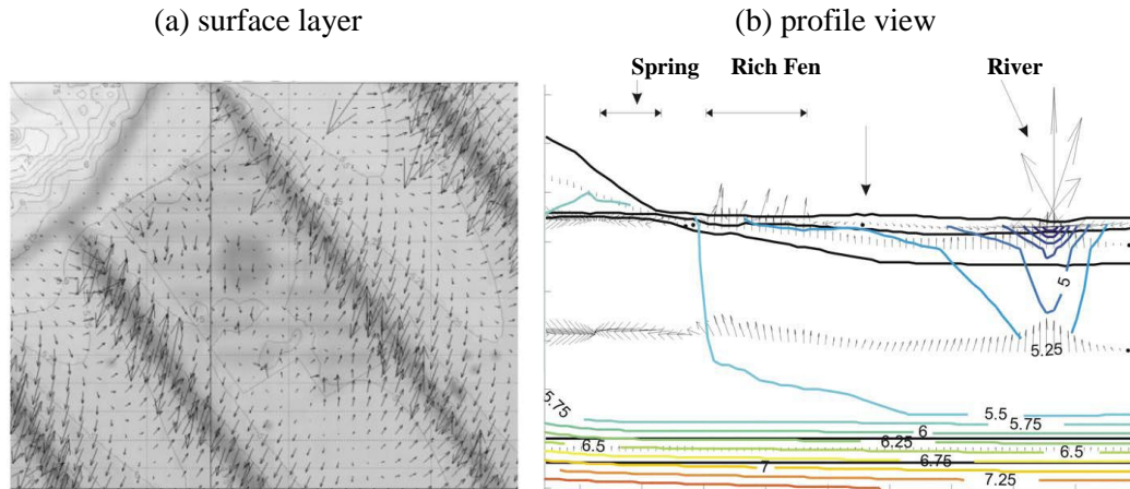
Fig. 9. Simulated flow vectors in the rich fen area. (a) Flow vectors in the surface layer (peat). (b) A profile view through all layers of the model. The position of the profile is similar to the profile in Fig. 7 .
