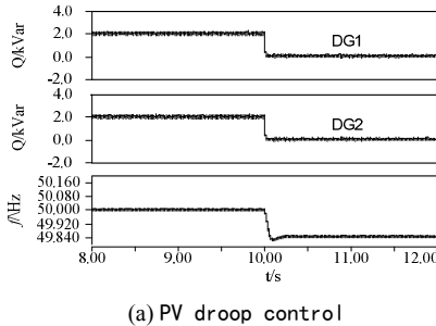
(a) PV droop control
