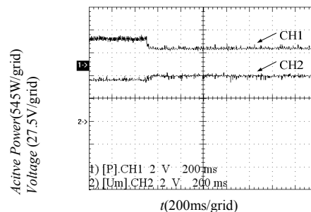
Fig.13 The output active power and the voltage of inverter while disconnecting to grid
