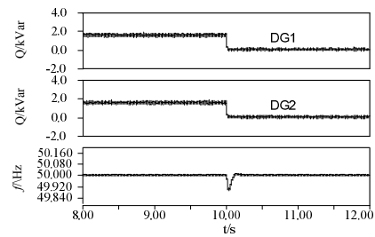
Fig.12 The output reactive power of inverters and the frequency of A point while disconnecting to grid
