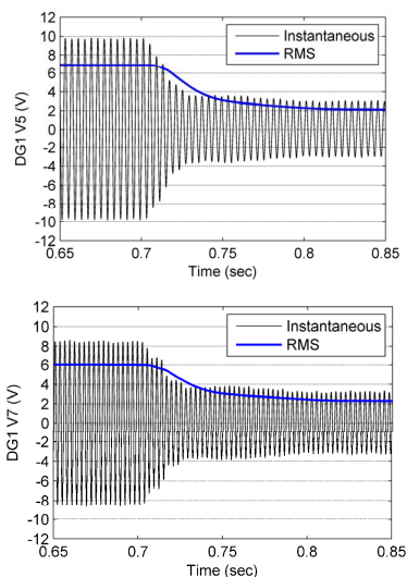
Fig. 10. 5 th and 7 th voltage harmonics of DG1
