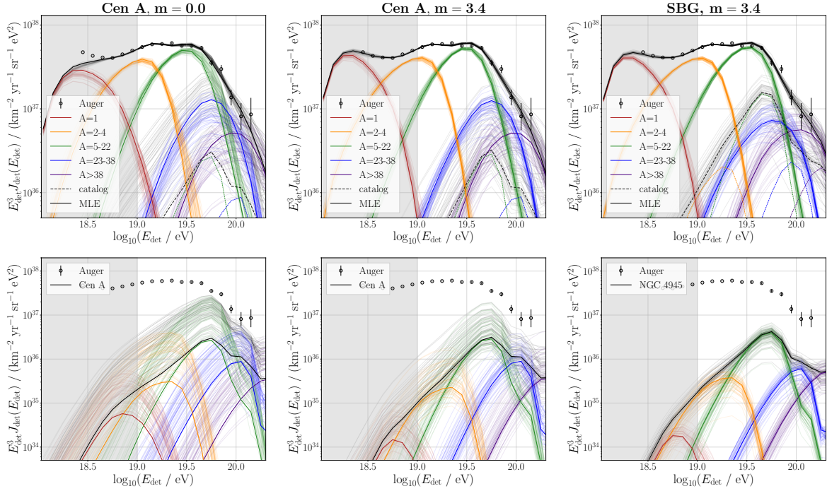
Figure 2. Modeled spectra on Earth for the Centaurus A model with m = 0 ( left ), with m = 3.4 ( middle ) and the SBG model with m = 3.4 ( right ). In this and all following figures the thick lines indicate the best-fit and the thin lines are drawn from the posterior distribution demonstrating the uncertainty. The markers represent the measured data of the Pierre Auger Observatory. The grey area symbolizes the energy bins which are not (fully) included in the fit (see section 3.1.2). In the upper row the total spectrum is depicted with the different element contributions in different colors. The contribution by the source catalog is indicated by the dashed line. The lower row shows the individual spectrum of the strongest source in the respective catalog.
