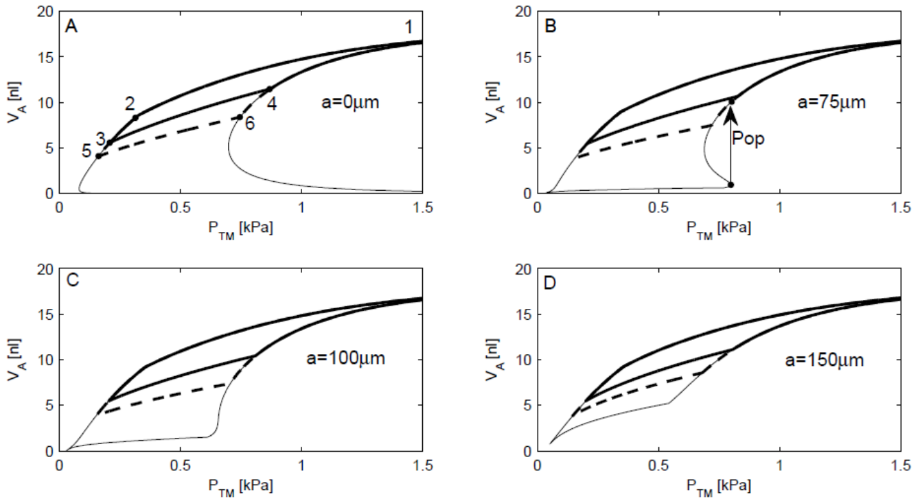
Fig. 16 The simulated PV -relationship of an alveolus including the mechanical properties of the tissue elasticity and surfactant. The bold line is a simulation with alveolar volumes ranging from TLC to FRC and back. The bold dashed line represents the physiological range of volume changes from TLC to RV . The lowermost line shows a simulation of compressions from maximum surface area to 5 %. In B the alveolus will “pop” open, once the transmural pressure exceeds the opening pressure of 0.8 kPa. The alveolar volume will suddenly increase as indicated by the arrow labeled Pop.
