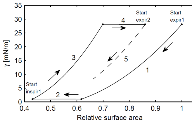
Fig. 14 Surface tension, \gamma , as a function of the relative alveolar surface area
