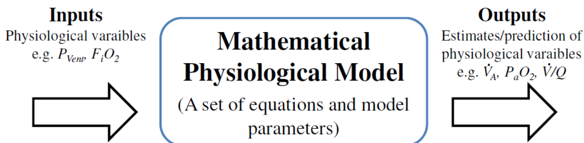
Fig. 9 A schematic diagram of the inputs and outputs to a mathematical and physiological model.
