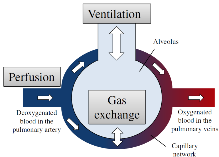
Fig. 2 Illustrates that gas-exchange in alveoli is a complex interaction between ventilation of air and perfusion of blood to the alveoli.
