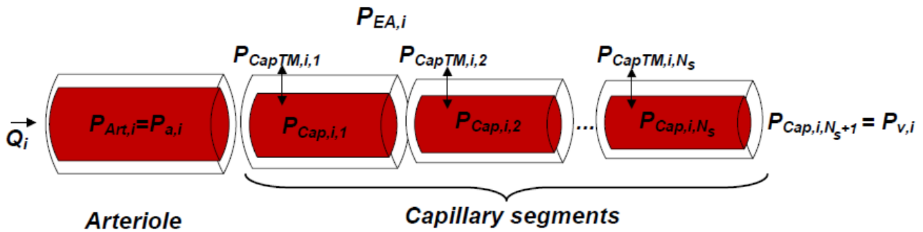
Fig. 29 Schematic representation of an arteriole and a capillary divided into segments each having a pressure drop. P_{EA,i} : Extraalveolar pressure. P_{a,i} : Arterial blood pressure. P_{v,i} : Venous blood pressure. Q_i : Blood perfusion. P_{CapTM,,i} : Capillary transmural pressure. P_{Cap,i,n} : Capillary pressure at layer i and segment n . P_{Art,i} : Arteriolar pressure.
