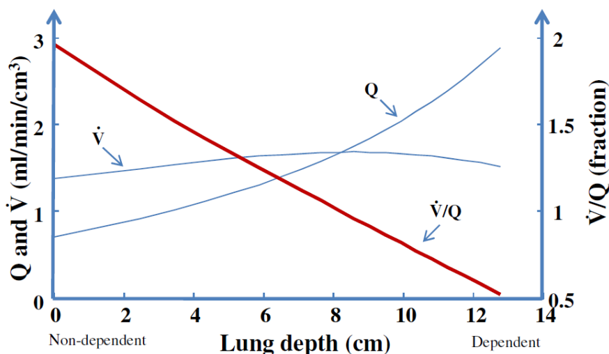
Fig. 8 Shows model simulated distribution of ventilation ( \dot{V} ) and perfusion ( Q ) and \dot{V}/Q -ratio from non-dependent to dependent part of the lungs similar to the one observed by West and his colleagues in the 1960's [44, 45].
