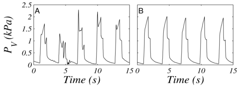
Fig. 22 Pressure measured by the ventilator, P_V , as a function of time. A: Pressure measurements of a subject participating in the ventilation. B: A fully relaxed subject not participating in the ventilation.
