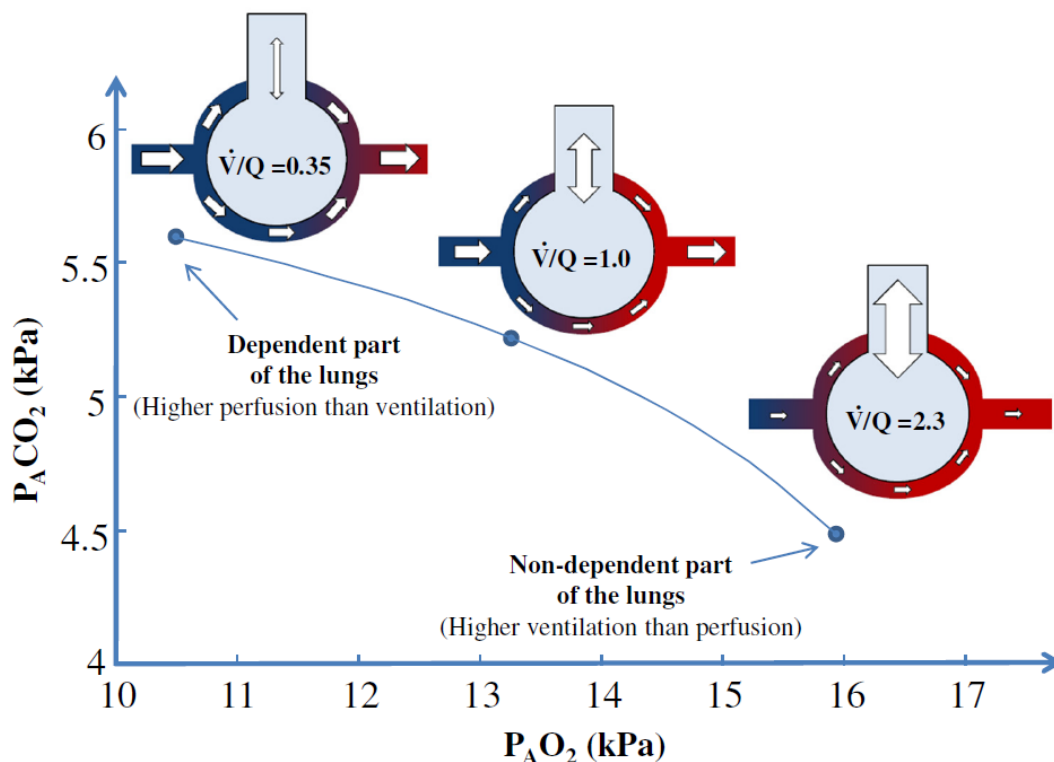
Fig. 3 Simulated relationship between alveolar partial pressure of O_2 and CO_2 for a healthy subject in upright position. Indicated is also the ventilation/perfusion ratio.
