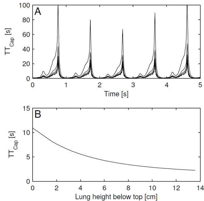
Fig. 28 A: Transition time during a tidal breath in layer number 1, 25, 50, 75 and 100 (most dependent, dashed line) and B: Mean transition time as a function of the lung depth.
