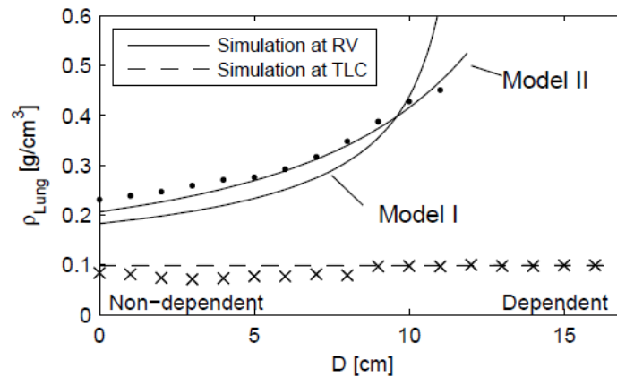
Fig. 20 Simulated density, \rho_{Lung} , related to lung depth, D , is shown at TLC (dashed line) and RV (solid line) for both models of the lung tissue elasticity. Data read from Millar and Denison [123] are shown for TLC and RV (crosses and dots, respectively).
