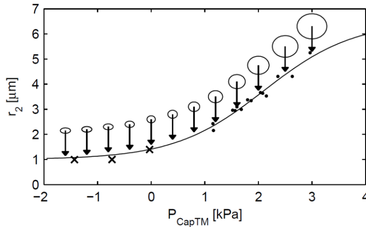
Fig. 25 The relationship between capillary transmural pressure and capillary radius. Data read from Sobin et al. [126] (dots) and Glazier et al. [127] (crosses) are illustrated. A sigmoidal curve has been fitted to the data points. The shapes of the capillaries are indicated at different transmural pressures.
