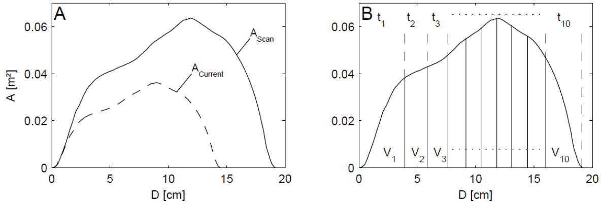
Fig. 18 A: The relationship between the cross sectional area, A , and lung depth, D , at total lung capacity of 6.8 l (solid line) and at 3 l (dashed line). B: The distribution of volume in layers when the lungs are divided into 10 layers. The thickness, t_i , and volumes, V_i , of each layer are also illustrated.
