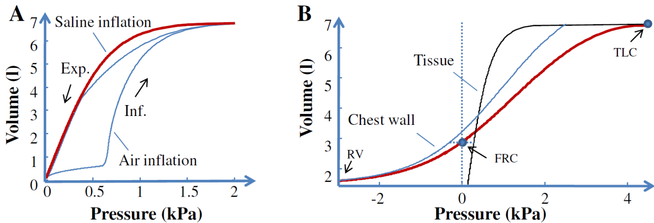
Fig. 4 A: Illustrates simulated pressure-volume relationship of an isolated lung inflated with saline (red line) or air (blue line). B: Simulated total pressure-volume curve (red line) including the effect of chest wall (blue line) and lung tissue elasticity (black line). RV : Residual volume. FRC : Functional residual capacity. TLC : Total lung capacity.
