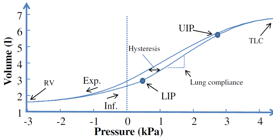
Fig. 5 Shows a simulated total pressure-volume curve from residual volume ( RV ) to total lung capacity ( TLC ) of a healthy subject. Indicated is the lung hysteresis, lung compliance, upper inflection point ( UIP ) and lower inflection point ( LIP ).
