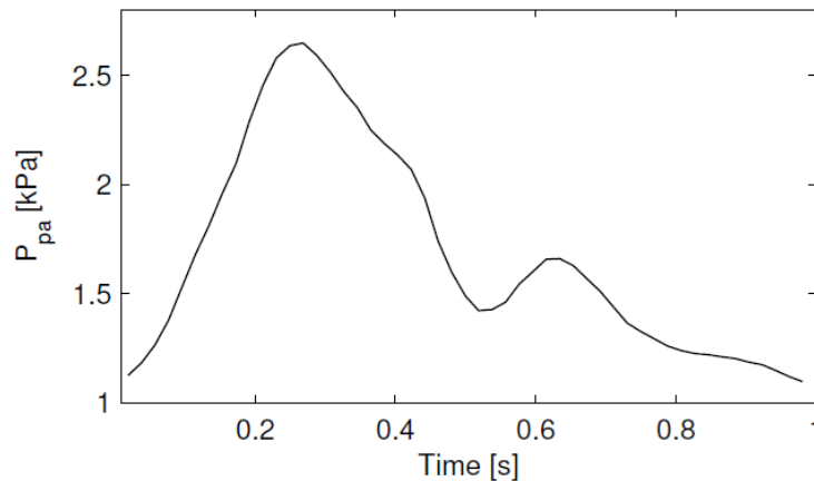
Fig. 26 The pulmonary pressure proximal to the capillaries at the height of the pulmonary valve, P_{pa} . The profile is shown for one heartbeat [128] scaled into the pressure range for pulmonary capillaries [61, 67].
