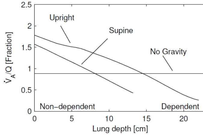
Fig. 32 Simulation results of ventilation-perfusion distribution down the lungs for a subject in upright, supine and with no gravity.
