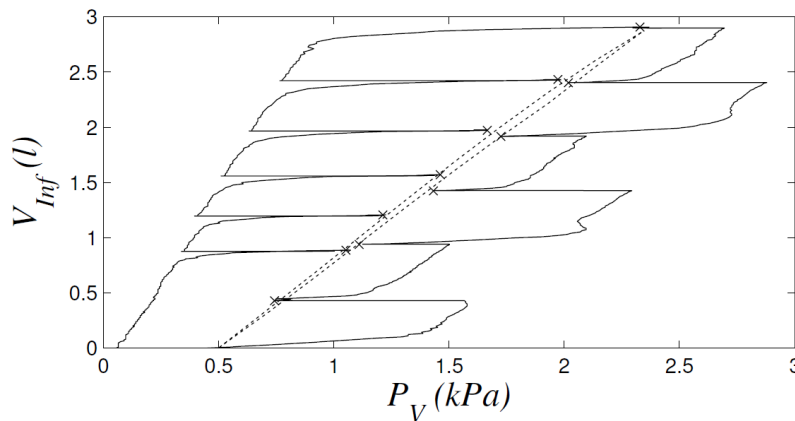
Fig. 23 Measured pressure-volume relationship from subject number 2. Crosses indicate the measured static pressure-volume points. Dotted line shows a simulated static pressure-volume curve using the identified parameters.
