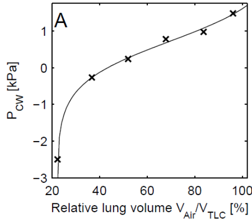
Fig. 17 The relationship between total lung volume and pressure exerted by chest wall. Data (crosses) read from Konno and Mead [121].
