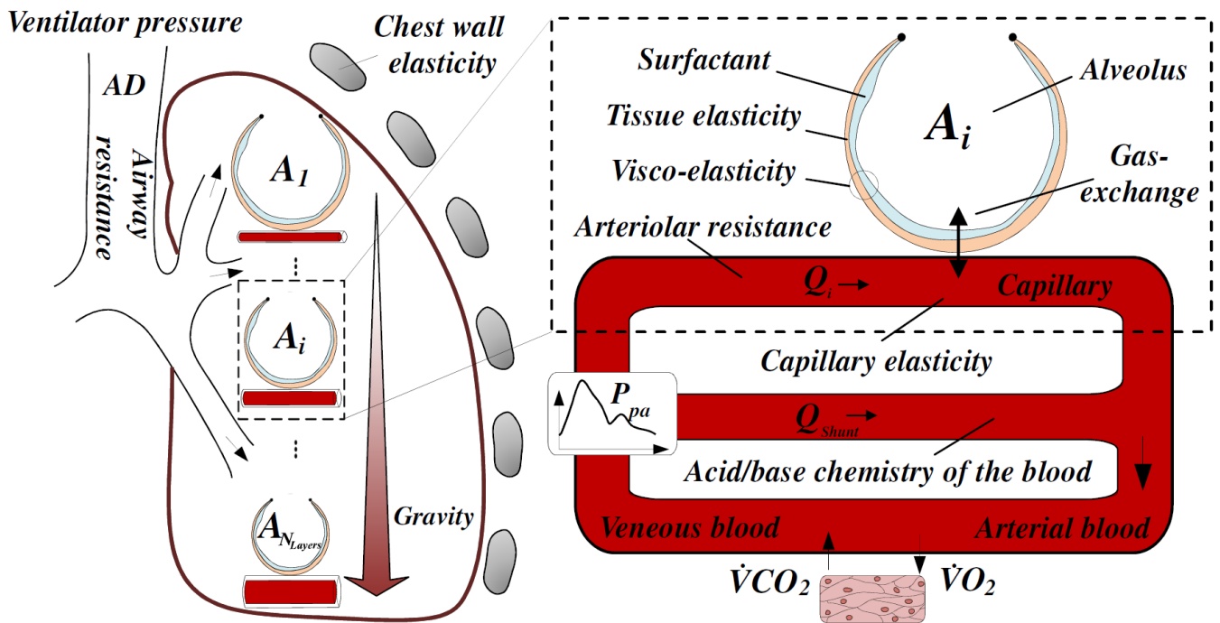
Fig. 10 Illustration of model components included in the total lung model. The lungs are divided into a number of horizontal layers, N_{Layers} . Shown are the anatomical dead space, AD , alveoli at layer i , A_i , capillaries, arterial and venous blood. Physiological components included are the ventilator pressure, airway resistance, gravity, chest wall elasticity, surfactant, tissue elasticity, viscoelastic properties of the lungs, gas-exchange, arteriolar resistance, capillary elasticity, pulmonary arterial pressure, P_{pa} , perfusion at layer i , Q_i , shunt, Q_{shunt} , acid/base chemistry of the blood, tissue elimination of CO_2 and consumption of O_2 , \dot{V}CO_2 , and \dot{V}O_2 .
