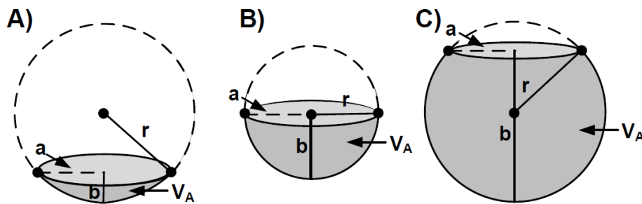
Fig. 12 Illustration of an alveolus, assuming that the circumference of the alveolar opening is constant. a : alveolar opening radius. r : radius of the alveolus. b : height of the alveolus.
