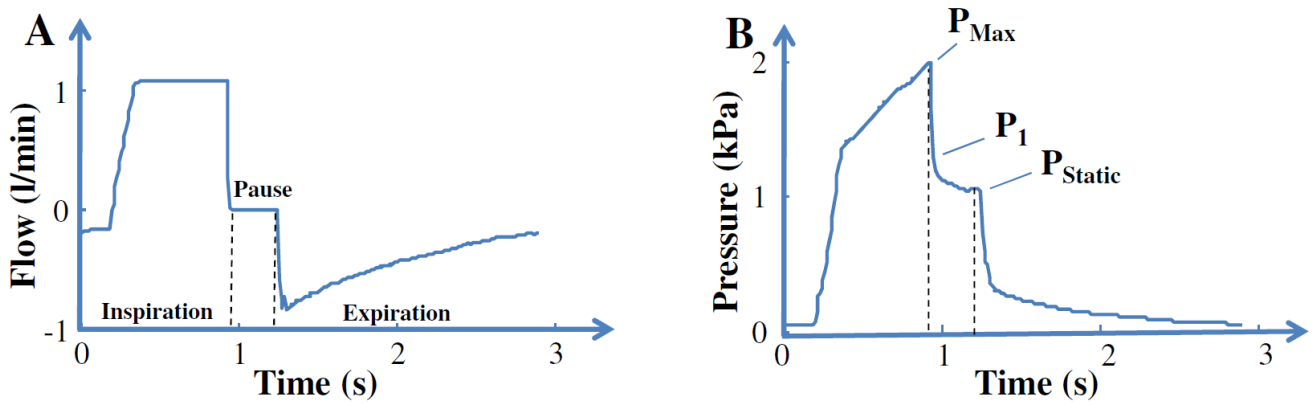
Fig. 6. Shows measured flow of gas (A) and pressure measured at the mouth (B) during a constant flow inflation, with a period of zero flow (pause) followed by a passive expiration [22]. During the pause period the airway pressure rapidly drops from its maximum value, P_{Max} , to P_1 , this is followed by a slower decrease to an apparent static plateau, P_{Static} .
