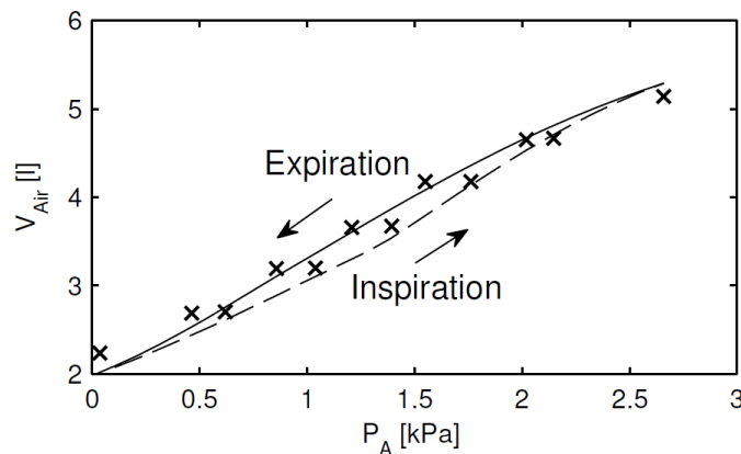
Fig. 19 The static pressure-volume relationship during a simulation with an alveolar pressure range between 0 and 2.66 kPa. PV -measurements by Sharp et al. [49] (crosses) are also shown. Dashed and solid lines indicate inspiration
