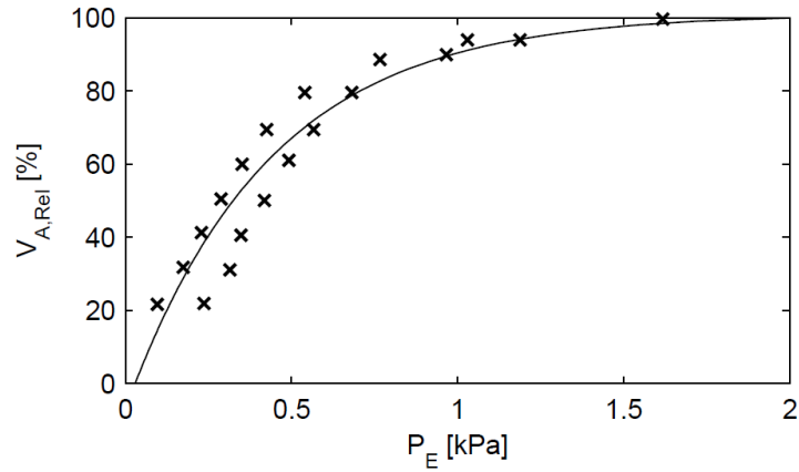
Fig. 13 The model (curve) of recoil pressure, P_E , exerted by the tissue of an alveolus and the volume of the alveolus. Data (crosses) have been read from Smith and Stamenovic [37].
