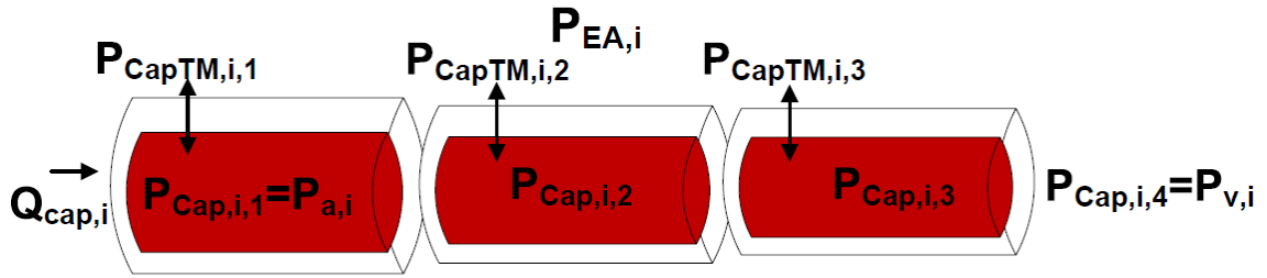
Fig. 24 Schematic representation of the capillaries divided into three segments each having a pressure drop. P_{EA} : Extraalveolar pressure. P_a and P_v : Arterial and venous blood pressure. Q : Blood perfusion. P_{CapTM} : Capillary transmural pressure. P_{Cap} : Capillary pressure
