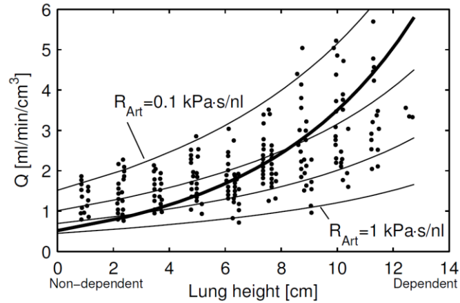
Fig. 30 Simulation results of the sensitivity analysis on R_{Art} . Perfusion distribution is shown as a function of lung height. Thick line shows simulation similar to one described in Fig. 27. Indicated on the figure are simulation results of arteriolar resistances of 0.1 kPa · s/nl and 1 kPa · s/nl. In between are simulation results of arteriolar resistances of 0.25 kPa · s/nl and 0.5 kPa · s/nl. Data are from Brudin et al. [74] (dots).
