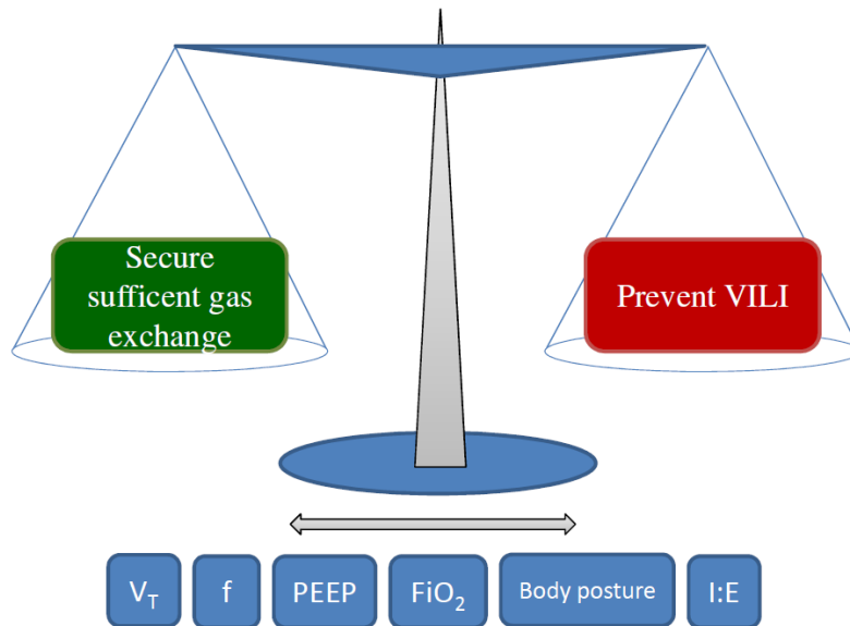
Fig. 1 Shows the tradeoff between ensuring sufficient gas-exchange while avoiding ventilator induced lung injury (VILI) when mechanically ventilating critically ill patients. Blue boxes illustrate that doctors have to optimize different ventilator settings and body posture considering the balance between achieving sufficient gas-exchange and preventing VILI. V_T : Tidal volume. f : Breathing frequency. PEEP : Positive end-expiratory pressure. F_iO_2 : Inspired oxygen fraction. I:E : Ratio between inspiration and expiration time.
