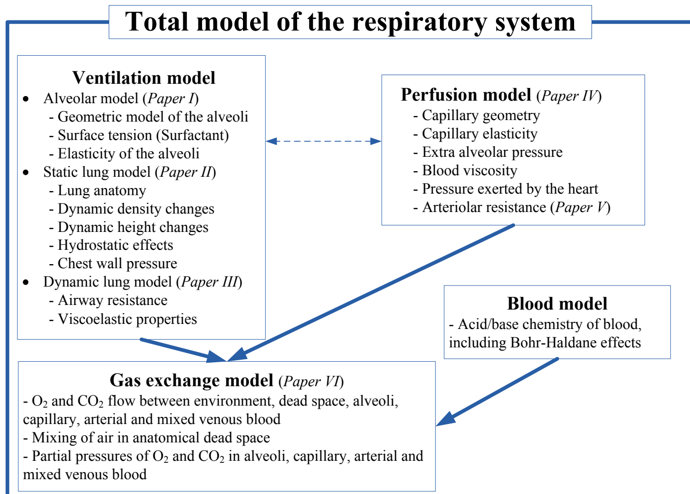
Fig. 11 The lung model is composed of four sub models i.e. a model of pulmonary ventilation, a model of pulmonary perfusion, a model of blood acid/base-chemistry and a model of gas-exchange. The sub models each include a number of physiological components that are listed in the model boxes. In the figure it is also indicated in which paper the different parts of the models are described. The dashed arrow shows the link between the ventilation model and the perfusion model through the extra alveolar pressure and the effect of capillary blood on lung density. The full arrows indicate that the gas-exchange model incorporates the other three sub models.
