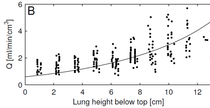
Fig. 27 Simulation of the perfusion (solid line) calculated as ml per minute per \text{cm}^3 lung parenchyma (including air) along with data read from Brudin et al. [74] (dots).
