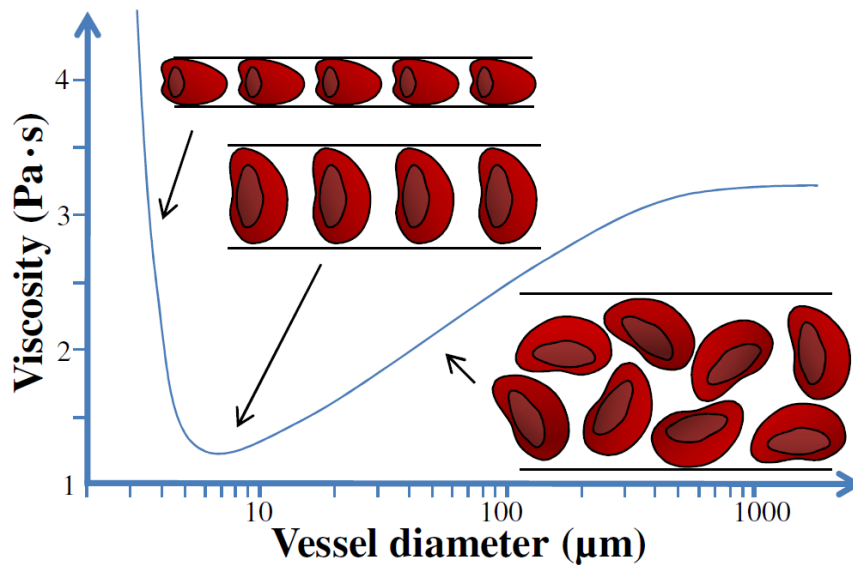
Fig. 7 Illustrates the viscosity as a function of vessel diameter for blood with a hematocrit of 45% simulated with a model by Pries et al. [71]. Illustrations of the blood flowing from left to right through tubes with different diameters.
