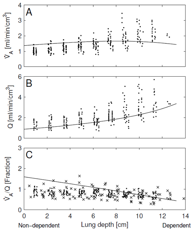
Fig. 31 A: Simulated alveolar ventilation calculated per \text{cm}^3 lung tissue (line) for a subject in the supine position and data measured by Brudin et al. [74] (dots). B: Simulated perfusion per \text{cm}^3 lung parenchyma (line) and data measured by Brudin et al. [74] (dots). C: Simulated ventilation-perfusion distribution according to lung depth and data measured by Brudin et al. [74] (dots) and Rhodes et al. [76] (crosses).
