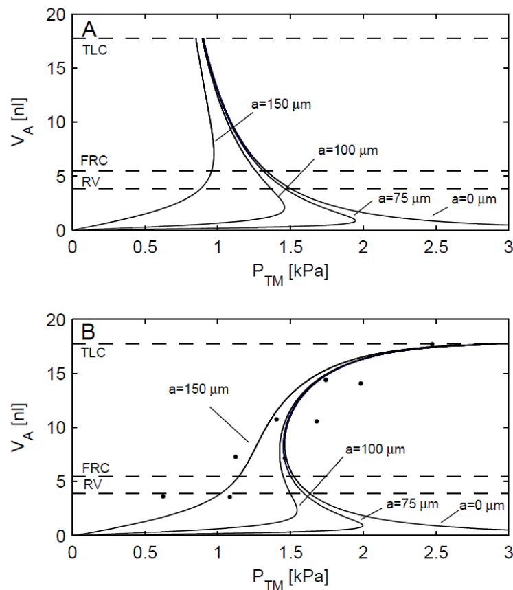
Fig. 15 A: PV -curves for an alveolus without surfactant and tissue elastic properties. B: Simulations of the alveolar PV -curve including the effects of tissue elastic properties and a surface tension of 73\ \text{mN/m} . The radius of the rigid ring a , varies between 0\ \mu\text{m} , 75\ \mu\text{m} , 100\ \mu\text{m} and 150\ \mu\text{m} . Experimental data indicated by dots [119]. The dashed lines indicate RV , FRC and TLC if all alveoli in the lungs were assumed to be identical.
