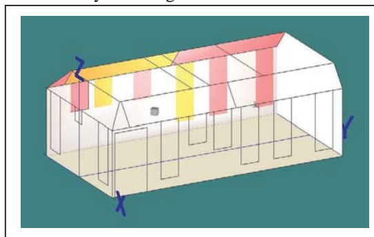
Figure 2. 3D CAD model of the standard listening room: surfaces with different material properties
