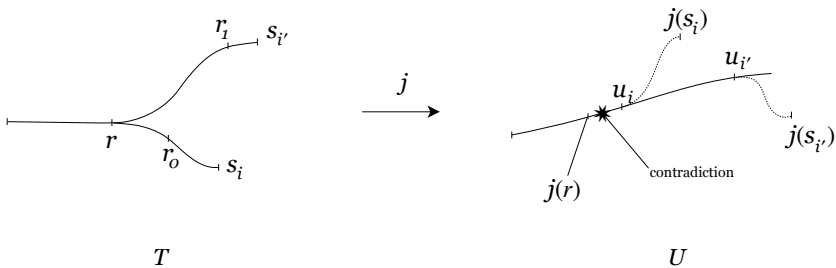
Figure 1. Contradiction assuming s_i \perp s_{i'} .
