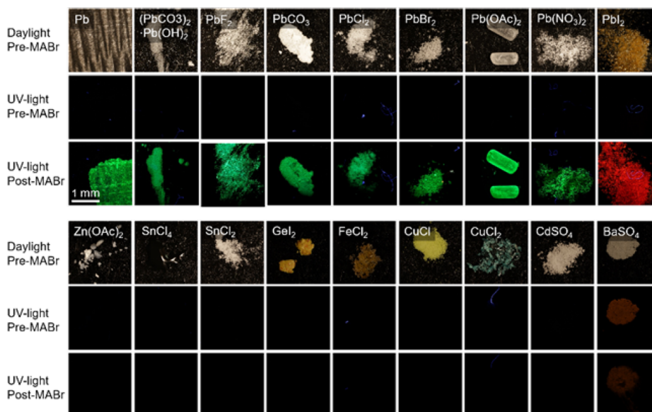
Figure 3. Chemosensitivity of photoluminescent lead detection: Selection of lead-containing, and lead-free samples before conversion under daylight, UV-light, and after spraying with the \text{CH}_3\text{NH}_3\text{Br} reagent, showing that all lead-containing samples show PL after conversion, while none of the lead-free samples show PL (an extensive list of more than 50 compounds is given in the Supporting Information). Lead-containing samples with halides can cause color shifts in the PL signal ( \text{PbF}_2 blueish, \text{PbI}_2 red).
