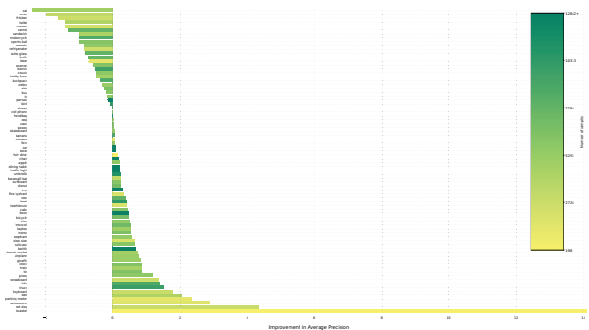
Figure 3. AP improvement per class. RP-FEM improves on two thirds of the classes in COCO over Mask R-CNN [12]. Classes with a low number of samples in the dataset particularly benefit from relational prior knowledge.
