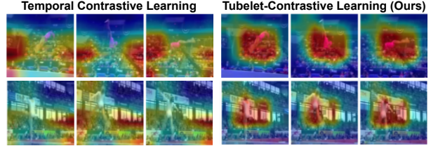
Figure 5: Class-Agnostic Activation Maps without Finetuning for the temporal contrastive baseline and our tubelet-contrast. Our model better attends to regions with motion.
