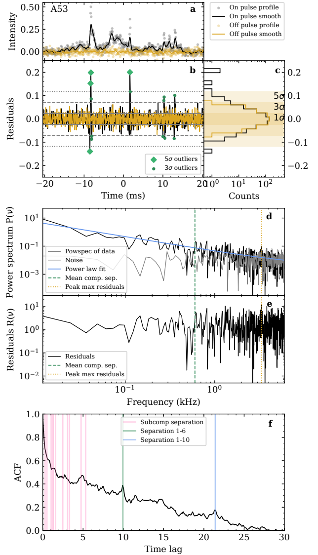
Fig. 5. Timing analysis of burst A53 from FRB 20180916B. Panel (a) shows the pulse profile of A53 as grey dots at 82 \mu\text{s} time resolution, and the smoothed profile as a black solid line. The yellow dots and solid line show the same for the off-burst signal. Panel (b) shows the residuals of the on- and off-burst signal as black and yellow lines, respectively. Green diamonds and dots show respectively the 5\sigma and 3\sigma outliers of the on-burst residuals. Panel (c) shows the distribution of the on-burst residuals in black and off-burst residuals in yellow. The yellow shaded regions, from dark to light, indicate the 1\sigma , 2\sigma , and 3\sigma contours of the off-pulse distribution fitted to a Gaussian. Panel (d) shows the power spectrum of A53 in black fitted to a power-law function shown in blue. The green dashed and yellow dotted lines mark the position of the mean component separation and the maximum of the residuals, respectively. Panel (e) shows the power spectrum residuals R(\nu) . Panel (f) presents the ACF of the light curve of A53 as a solid black line. The pink vertical lines indicate the separation between consecutive components, the green line the separation between the two brightest components, and the blue line the separation between the first and third brightest components.
