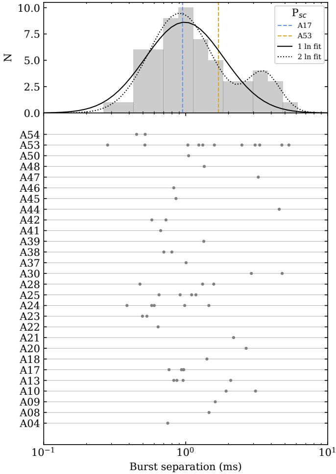
Fig. 4. Subcomponent separation of FRB 20180916B multi-component bursts presented in Pastor-Marazuela et al. (2021) . The top panel shows a histogram of the burst separation between discernible subcomponents in multi-component bursts. The mean A17 and A53 separations are shown as vertical dashed blue and yellow lines, respectively. The fit to a single lognormal and a double lognormal distribution are shown as solid and dotted black lines, respectively. The bottom panel shows the burst separations in each burst of the sample.
