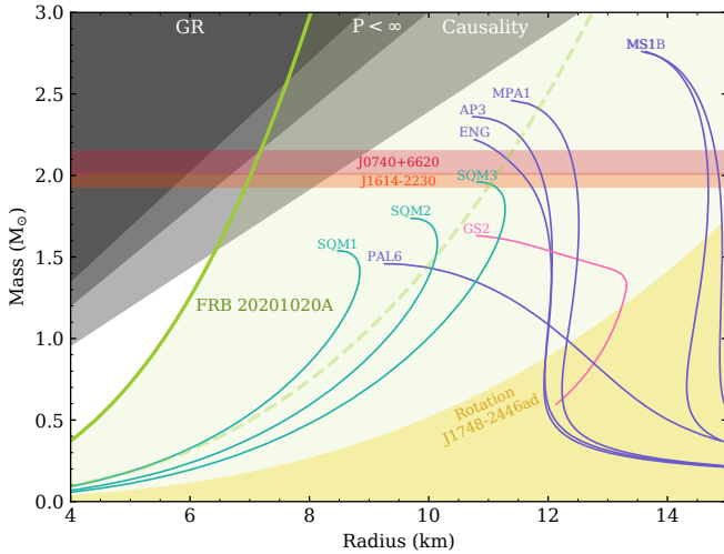
Fig. 6. Neutron star mass–radius diagram. The solid lines represent the mass–radius relationship of typical EoSs. The grey shaded regions are forbidden by general relativity, finite pressure ( P < \infty ), and causality. The yellow shaded region is forbidden by the rotation of the fastest spinning pulsar J1748–2446ad (Hessels et al. 2006). The red shaded region shows the mass of J0740+6620 (Cromartie et al. 2020; Fonseca et al. 2021) and the orange region the mass of J1614-2230 (Demorest et al. 2010), the two heaviest known NSs. Valid EoSs need to cross those regions. The green line and green shaded region would be forbidden if the quasi-period of FRB 20201020A were produced by the rotation of a NS at 2435 Hz, and the region to the right of the dashed green line would be forbidden if the rotation was at 1205 Hz.
