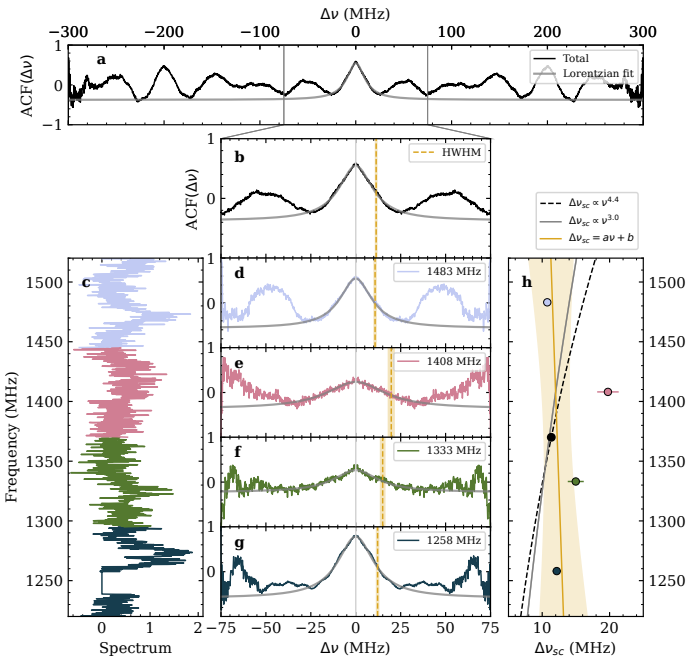
Fig. A.1. Scintillation analysis of FRB 20201020A. Panel (a) shows the ACF of the full spectrum of the FRB in black, with a grey solid line showing the fit of the central peak to a Lorentzian function. Panel (b) shows a zoomed-in version of the central 75 MHz of the ACF, with a yellow dashed line with shaded regions indicating the HWHM of the fitted Lorentzian. Panel (c) shows the spectrum of the FRB, with four different colours indicating the four sub-bands it was divided into. Panels (d), (e), (f), and (g) show the ACF of each of the four subbands of the spectrum, with colours matching the division of the spectrum, and the grey lines showing the fit of the central peak to a Lorentzian. The yellow dashed line with shaded contours marks the position of the HWHM. Finally, panel (h) gives the HWHM of each sub-band as a function of frequency. The coloured markers match the colours of the subbands, and the black marker indicates the HWHM over the whole spectrum. The black dashed line indicates the expected evolution with frequency for a power-law index \alpha = 4.4 , as expected from scintillation in the ISM. The grey line marks the fit of the four sub-band HWHMs to a power-law function, and the yellow line marks its fit to a linear function.
