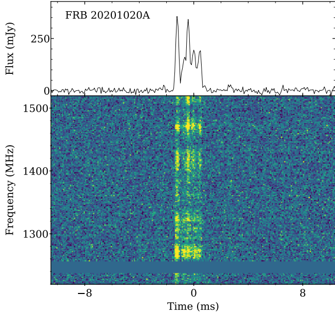
Fig. 1. Dynamic spectrum of FRB 20201020A, de-dispersed to a DM of 398.59 \text{ pc cm}^{-3} . The top panel shows the average calibrated pulse profile of the burst, and the bottom panel the intensity of the burst in time versus frequency. The data have been downsampled in frequency by a factor 8.
