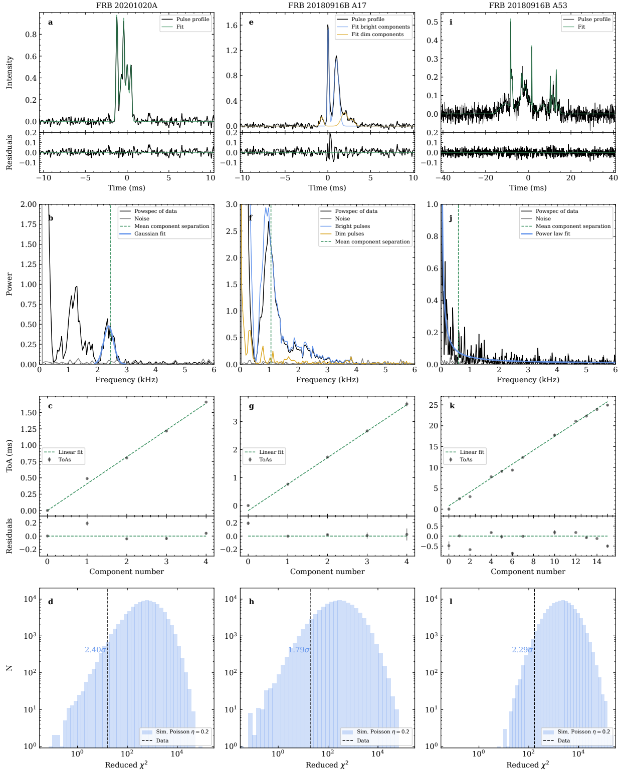
Fig. 3. Timing analysis of FRB 20201020A (left column), A17 (central column), and A53 (right column). The top of panels (a), (e), and (i) shows the pulse profile of each burst (black) and the fitted multi-component Gaussians in green for FRB 20201020A and A53; for A17 the bright components are shown in blue and the dim components in yellow. The bottom of panels (a), (e), and (i) shows the residuals of the multi-component Gaussian fit of each pulse profile. Panels (b), (f), and (j) show the power spectra of each pulse profile in black. In (b), the vertical dashed line indicates the average separation of the FRB 20201020A components, while the blue line shows the Gaussian fit to the 2.4 kHz component. In (f), the blue and yellow lines show respectively the power spectra of the bright and dim components. Panels (c), (g), and (k) show the ToAs of all subcomponents as a function of component number. In most cases, the error on the ToAs is smaller than the marker size. The dashed green lines in (c), (g), and (k) are linear fits to the ToAs, and the lower panels show their residuals normalised by the mean subcomponent separation P_{sc} . Panels (d), (h), and (l) show histograms of the simulated r\chi^2 statistic using a shifted Poissonian subcomponent spacing distribution with \eta = 0.2 to compute the significance of the periodicity. The vertical lines correspond to the r\chi^2 of the linear fit to the data. The significance is indicated as blue text.
