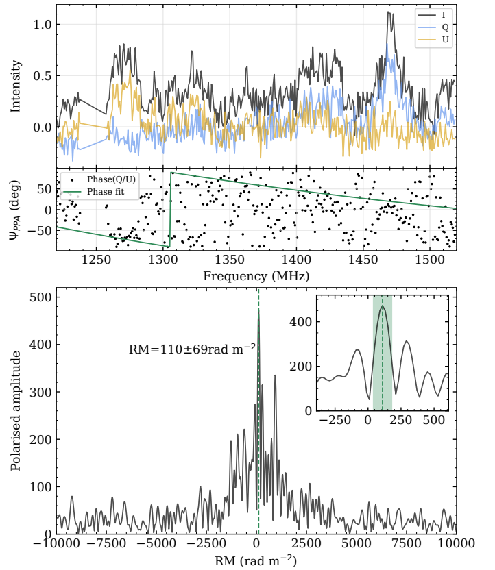
Fig. D.1. Measured polarisation properties of FRB 20201020A. The top panel shows the Stokes parameters I (black), Q (blue) and U (yellow) as a function of frequency, calibrated by assuming Stokes V to be zero. The second panel shows the measured phase between Q and U (black dots) and its fit in green. The bottom panel shows the RM-synthesis solution, with the polarised amplitude as a function of RM. The dashed green line marks the position of the maximum, at RM = +110 \pm 69 \text{ pc cm}^{-3} . The inset shows the same, but zoomed in at the central peak of the polarised amplitude.
