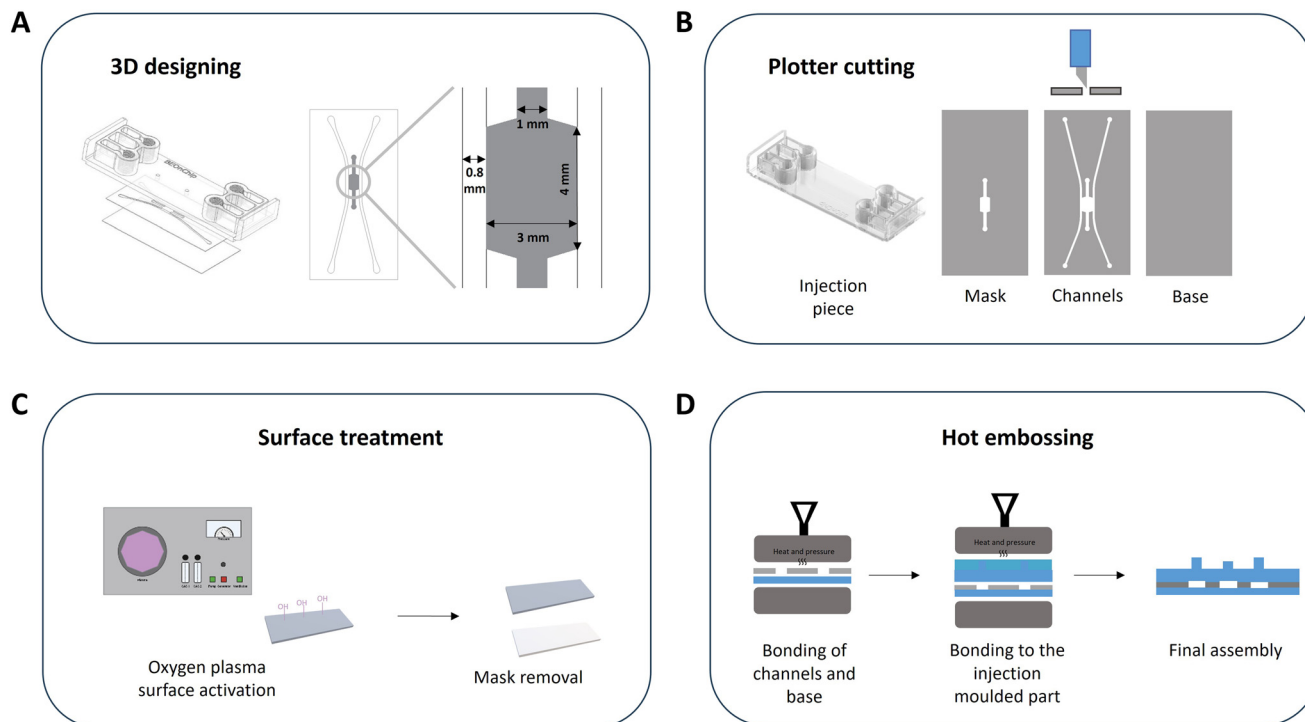
Fig. 1 Fabrication process. (A) Design of the device. 3D exploded model and 2D channel layer with details of the central chamber area. (B) Material selection and cutting. The design of olefin copolymers and plotter cutting is used to achieve the desired geometries. The design of the central channel is used to obtain the mask and the central and lateral channels. (C) Surface treatment. Oxygen plasma surface activation process using the mask with the central chamber geometry. (D) Thermocompression bonding. Firstly, the channel layer is bonded to the base; finally, channels are bonded to the injection piece.
