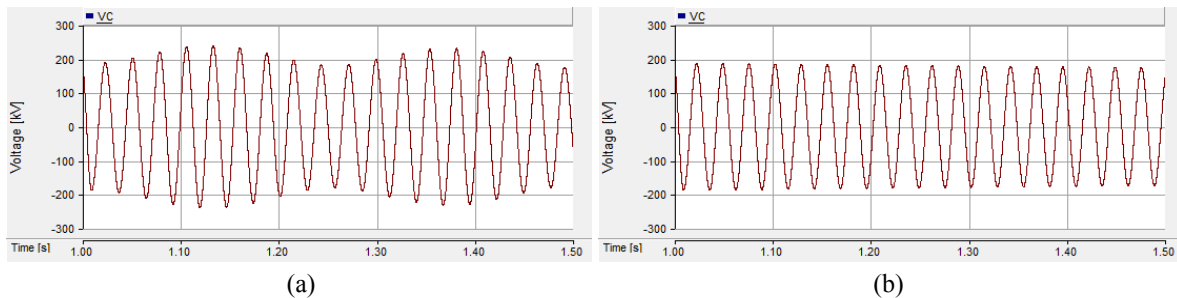
Figure 11.17 - Voltage after disconnection in Phase C. a) Example 1; b) Example 2
