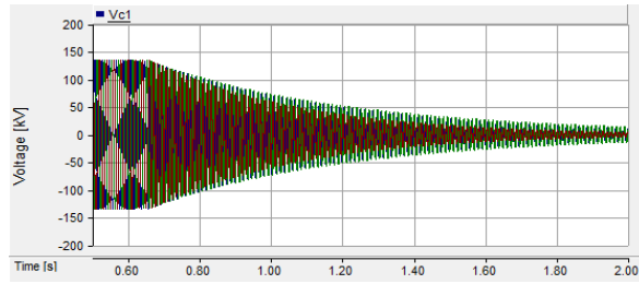
Figure 5.66 - Cable+Shunt Reactor disconnection – stable and accurate simulation
