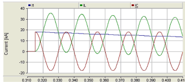
Figure 5.6 - Current in the inductor ( I_L ), in the capacitor ( I_C ) and the sum ( I_I = I_L + I_C )
