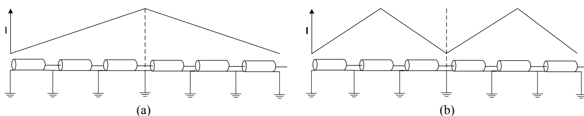
Figure 7.19 - Relative current along a cable with six major cross-bonded sections. a) 1st parallel resonance point ( \sim 4 kHz); 2nd parallel resonance point ( \sim 8 kHz)
