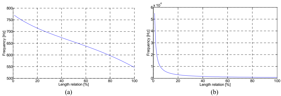
Figure 5.39 - Frequencies as a function of cable length for C=10.087\mu F and L=16.8mH (length of reference equal to 47.49km). a) First resonance frequency; b) Second resonance frequency
