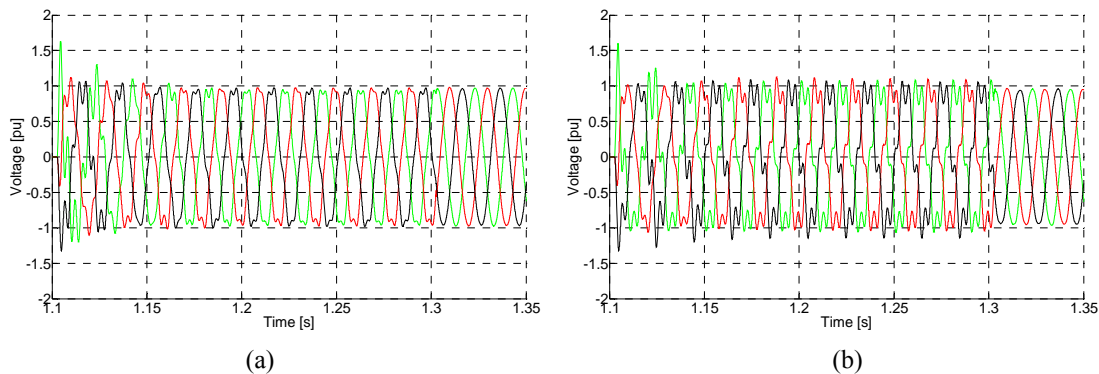
Figure 7.4 - Cable energisation with 5th harmonic excitation. a) Model D5-L; b) Model D3-L
