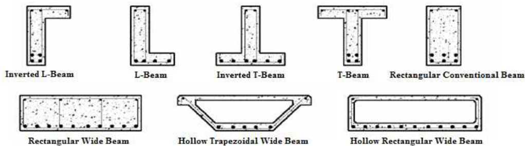
Figure 2: Types of Concrete Beams According to the shape of their Cross Section (Source: Al.Dywany, 2010).
