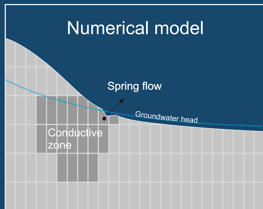
Figure 4: Principle of spring flow in the numerical model
