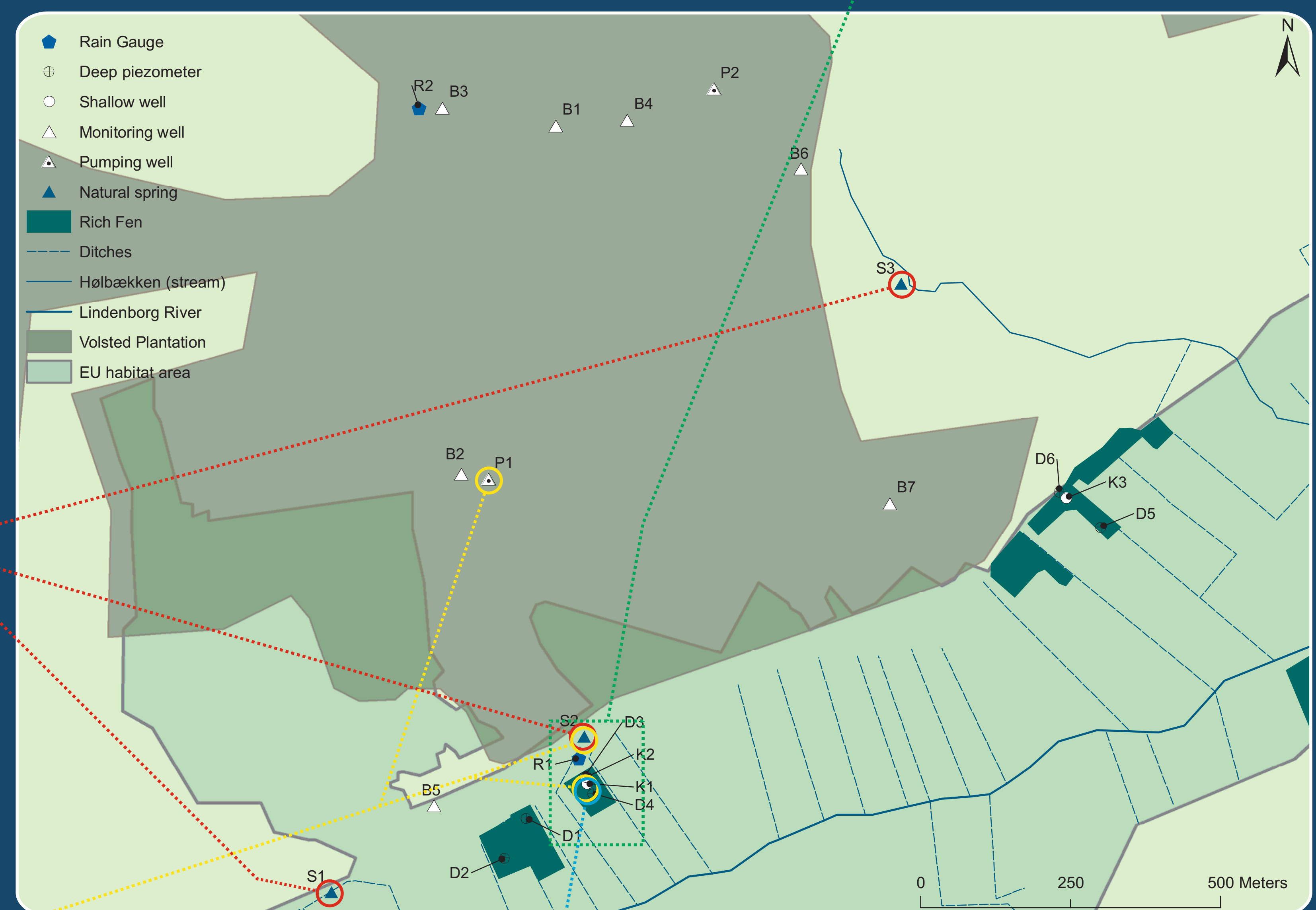
Figure 1: Boundary for the nested hydrological models
