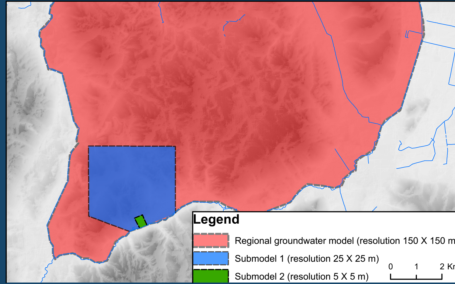
Figure 1: Boundary for the nested hydrological models
