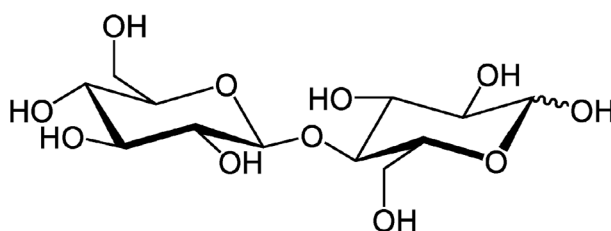
Figure 1: Molecular structure of cellobiose
