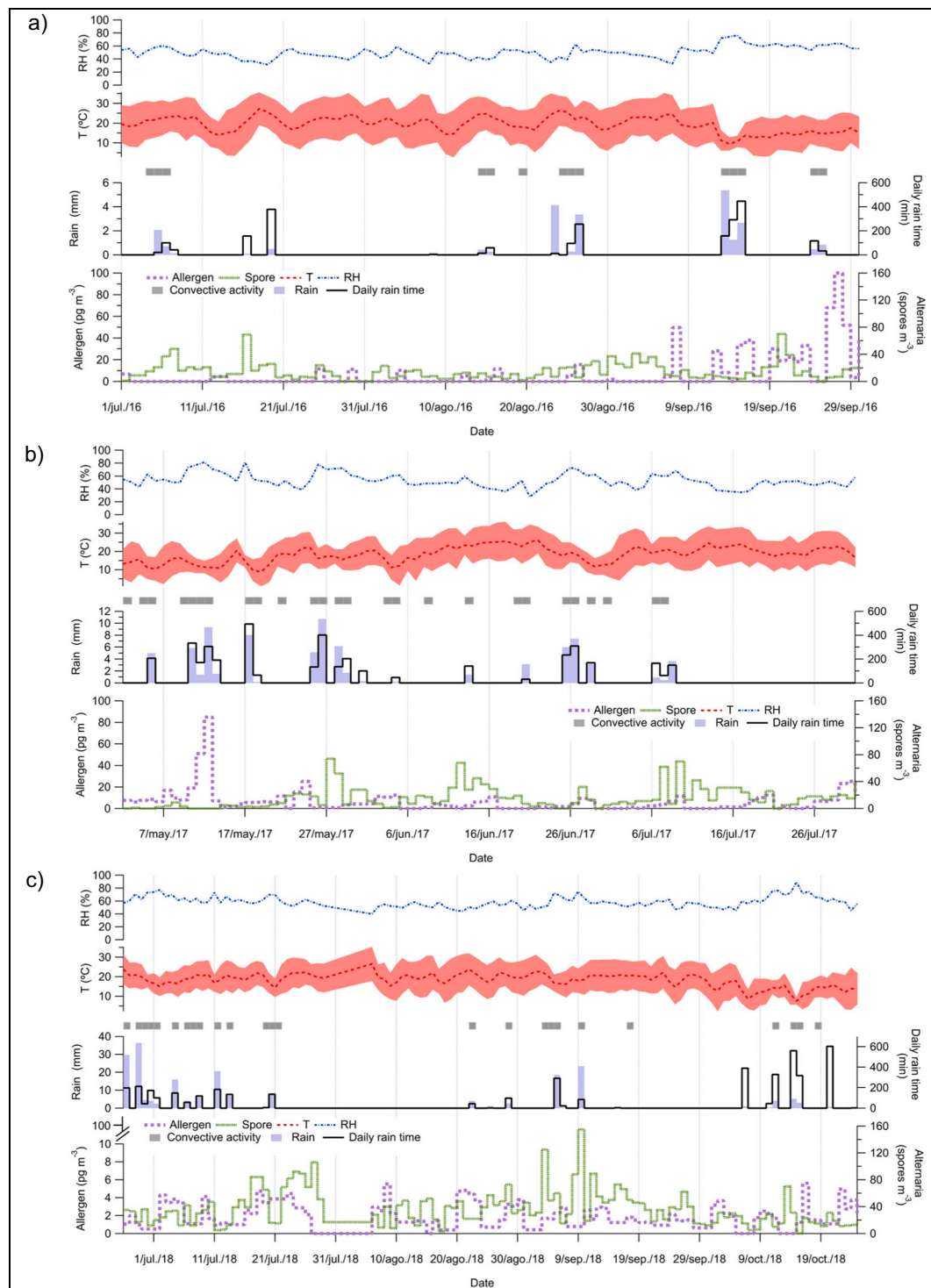
Fig. 3. Daily evolution of Alt a 1 allergen, Alternaria spores and meteorological variables during the sampling period in: a) 2016; b) 2017; c) 2018; d) 2019; e) 2020.
