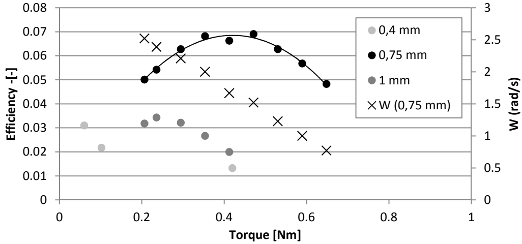
Figure 11. Efficiency depending on fin's thickness for different torque values under target wave condition 4 (RW4). 4 sets of fins, 6 fins per set, draft=0.36 m. Measured H=0.11 m, T=2 s.
