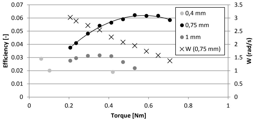
Figure 12. Efficiency depending on fin's thickness for different torque values under target wave condition 5 (RW5). 4 sets of fins, 6 fins per set, draft=0.36 m. Measured H=0.13 m, T=2.2 s.
