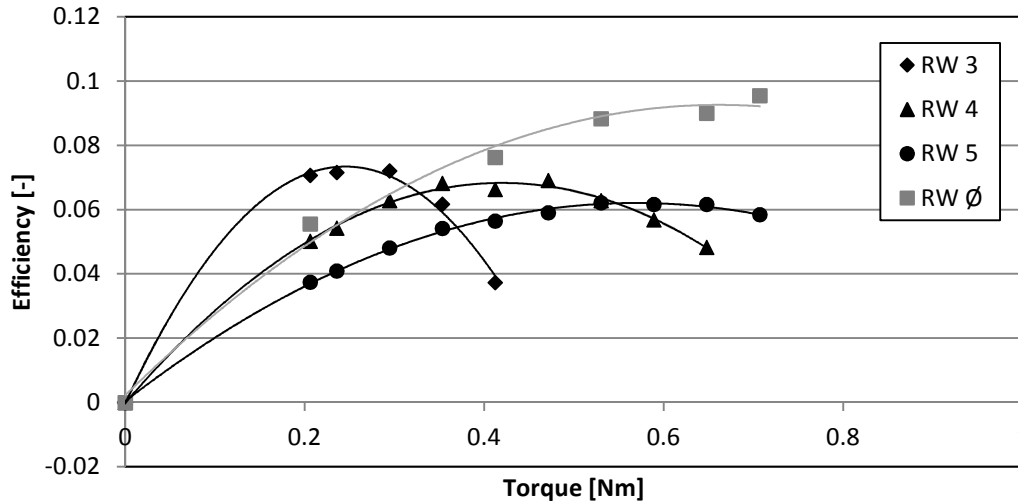
Figure 14. Best results. Comparison of results for different wave conditions, fin's thickness = 0.75 mm, 4 sets of fins, 6 fins per set.
