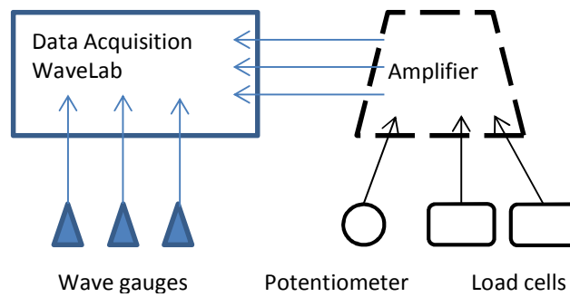
Figure 5. General scheme of the measuring system
