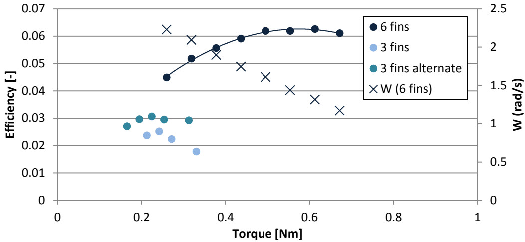
Figure 26. Efficiency for different no. of fins per set depending on torque values under wave condition 5 (RW5). 7 sets of fins, 0.75 mm thickness, 0.36 m draft. Average measured H=0.13 m, T=2.2 s.
