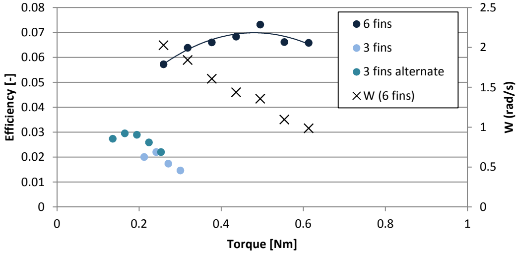
Figure 25. Efficiency for different no. of fins per set depending on torque values under wave condition 4 (RW4). 7 sets of fins, 0.75 mm thickness, 0.36 m draft. Average measured H=0.11 m, T=2 s.
