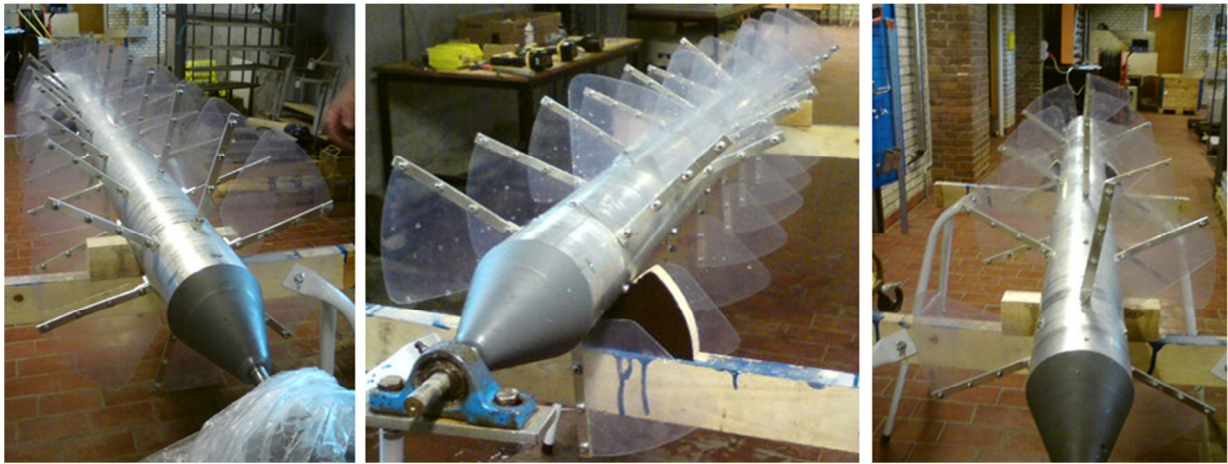
Figure 24. From the left to the right, short model equipped with 7 sets of fins, 6 fin's par set (lf), 3 fin's part set (c), 3 fin's par set-alternate (rg). Fin's thickness=0.75 mm.
