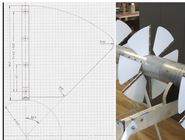
Figure 2. Fins' profile.
