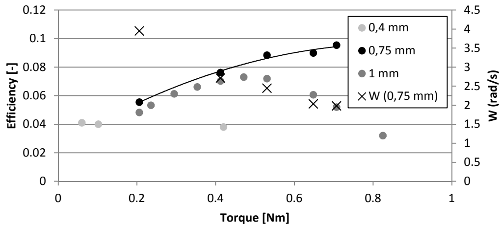
Figure 13. Efficiency depending on fin's thickness for different torque values under target wave condition \emptyset (RW \emptyset ). 4 sets of fins, 6 fins per set, draft=0.36 m. Average measured H=0.16 m, T=1.4 s.
