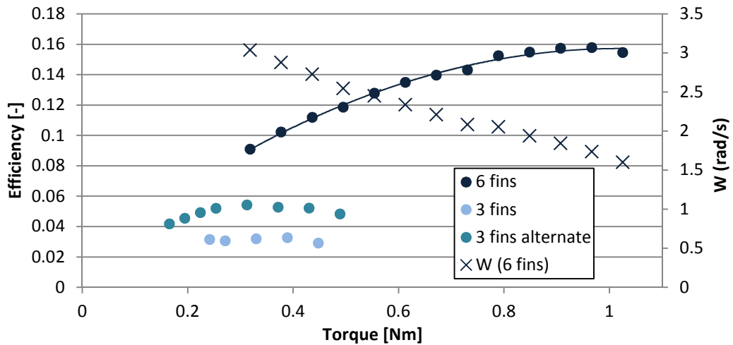
Figure 27. Efficiency for different no. of fins per set depending on torque values under wave condition \emptyset (RW \emptyset ). 7 sets of fins, 0.75 mm thickness, 0.36 m draft. Average measured H=0.14 m, T=1.4 s.
