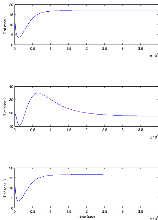
Fig. 3. Simulation results with a controller designed for the system with the fault-free actuator set: \{a, b, g, h, j\}
