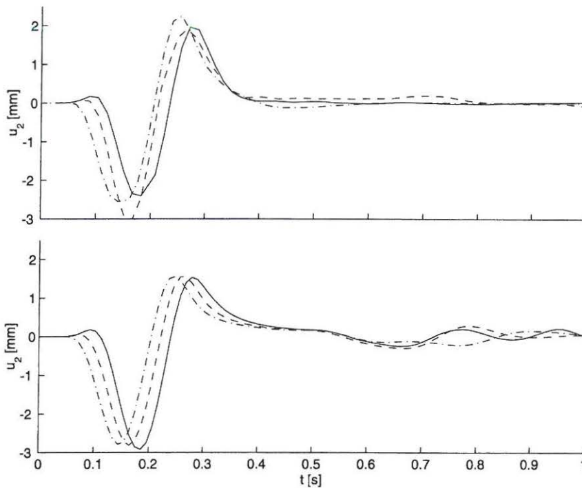
Fig. 10. Vertical displacements at (\bar{x}_1, \bar{x}_2, \bar{x}_3) = (-20 \text{ m}, 0 \text{ m}, 0 \text{ m}) obtained using BEM (top) and FEM (bottom) for v_1 = 0 (—), v_1 = 0.2c_s (---) and v_1 = 0.5c_s (-·-·-·).
