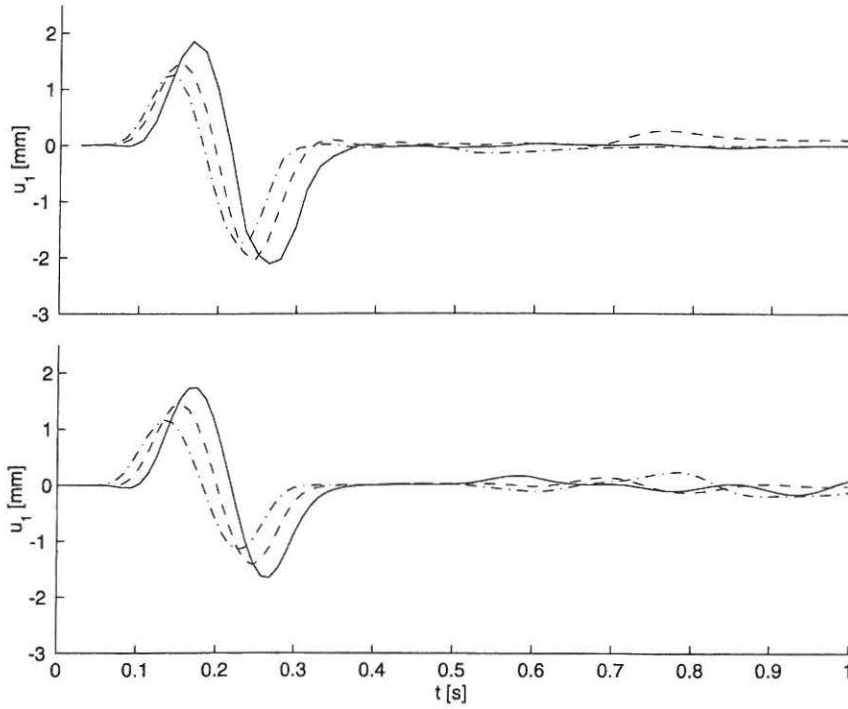
Fig. 9. Horizontal displacements at (\bar{x}_1, \bar{x}_2, \bar{x}_3) = (-20 \text{ m}, 0 \text{ m}, 0 \text{ m}) obtained using BEM (top) and FEM (bottom) for v_1 = 0 (—), v_1 = 0.2c_s (---) and v_1 = 0.5c_s (-·-·-·).
