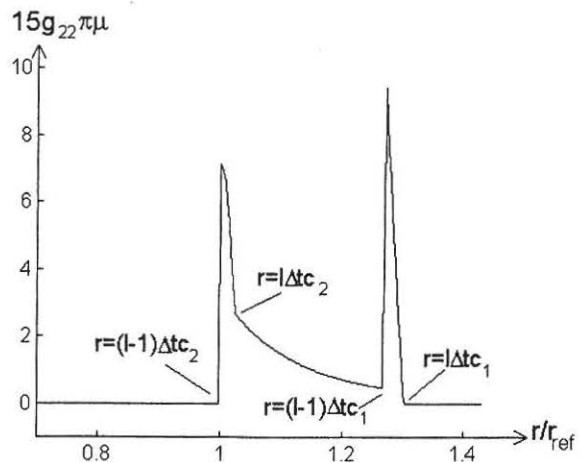
Fig. 3. Section of the wave front over which the integration is performed r_{ref} = (l - 1)\Delta tc_s .
