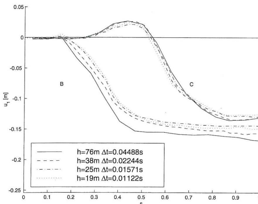
Fig. 4. Horizontal displacements at B: (\bar{x}_1, \bar{x}_2, \bar{x}_3) = (152 \text{ m}, 0 \text{ m}, 0 \text{ m}) , C: (\bar{x}_1, \bar{x}_2, \bar{x}_3) = (305 \text{ m}, 0 \text{ m}, 0 \text{ m}) .
