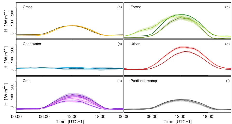
Figure 5. Average diurnal cycle of the sensible heat flux in the warm season of different land cover types, indicating a difference in sensitivity to environmental drivers. Each colored line represents a measurement site. The uncertainty, here defined as twice the standard error, is presented as the shaded area around the solid lines.
