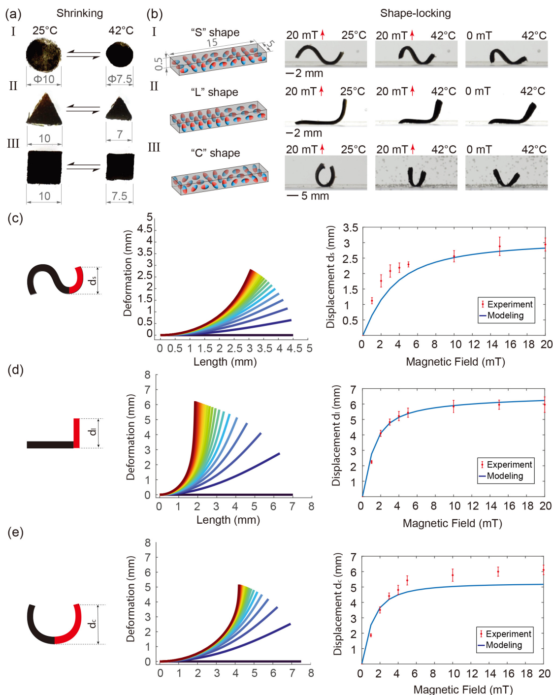
Fig. 4 Thermal-shrinking and shape-locking features of the dual responsive sheets. (a) Reversible thermal shrinking of different shapes, namely circular (I), triangular (II) and rectangular (III). The original dimensions are measured at room temperature (25°C), the shrunken dimensions are measured at completed shrinking point at 42°C as characterized. Dimensions are in mm. (b) Magnetic programming and shape-locking property of three typical geometry shapes are shown. The magnetization profile of each shape is indicated in the first column of figures. The red solid arrows indicate the direction of the applied magnetic field. Simulation results of deformation of the (c) "S", (d) "L" and (e) "C" shaped robot. The deformation of the right quarter of the robot under increased magnetic field strength from 0 mT to 20 mT is shown in the middle graph. Both experiment and simulation results of the displacement of the right tip are shown in the right graph.
