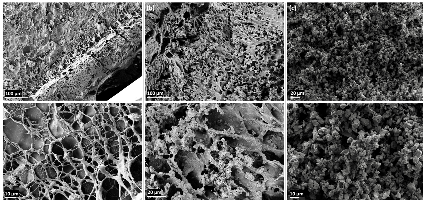
Fig. 2 SEM images depict (a) the cross-section of the NIPAM@Control sheet after freeze drying, (b) the cross-section of THANOS after freeze drying, showcasing a uniform dispersion of ferromagnetic particles within the hydrogel, and (c) ferromagnetic MQFP TM -16-7-11277 particles observed as a powder without being incorporated in a polymeric matrix.
