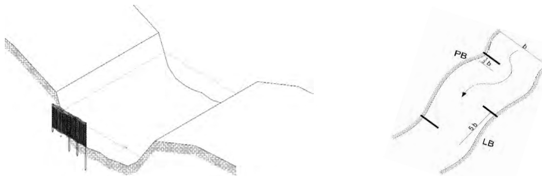
Fig. 1. The deflector scheme and placement along the studied section of the Flinta River: a) completed deflector in the river; b) scheme of the location of deflectors in the river.
