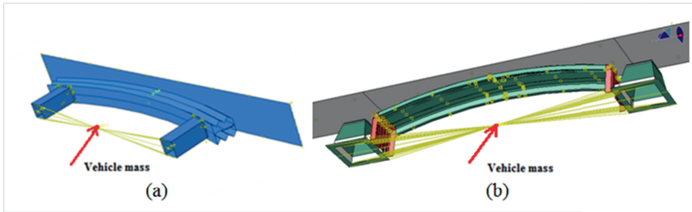
Fig. 1. Simplified FEM bumper models: a – pultruded beam solution, b – die forming integrated beam – crash box solution
