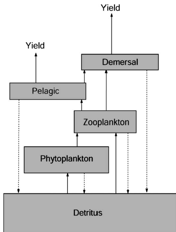
Figure 2. Trophic interactions between five components of the southern Benguela ecosystem (adapted from Mullon et al. , 2004).
