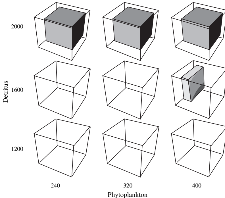
Figure 3. Viability kernel approximation to the southern Benguela ecosystem (grey; horizontal axis, zooplankton biomass; vertical axis, demersal fish biomass; depth, pelagic fish biomass; adapted from Mullon et al. , 2004) for different levels of detritus (ranging from 1200 to 2000 \text{t km}^{-2} ), and phytoplankton (ranging from 240 to 400 \text{t km}^{-2} ; for constraints see Table 1). Yields of pelagic and demersal fish are 3 and 2 \text{t km}^{-2} , respectively.
