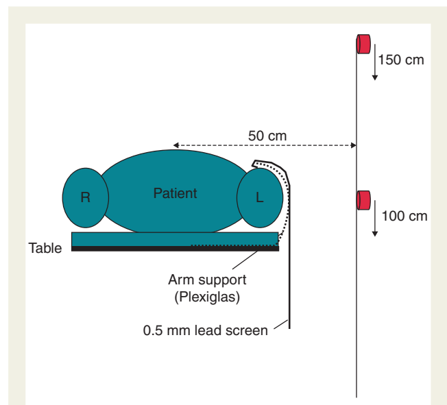
Figure 9 Optimization of the lead protection during device implantation procedures, Cross-sectional view of a patient on the fluoroscopy table. The operator usually stands on the left side of the patient and therefore the dose rates were measured at that side at 100 and 150 cm above the floor with the patients heart in the isocentre. The dosimeters are sketched in red. The custom 0.5 mm lead screen, made of 50 × 50 cm apron material, hangs on a custom Plexiglas arm support and shields both the upper part of the patients arm as well as the left side of the patient from the operator. That screen reduced the operator exposure with 22–94% depending on the projection angle and the measurement position (Table 6).
