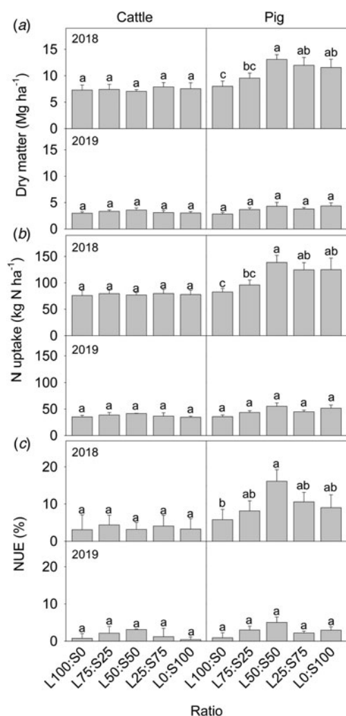
Fig. 4. Dry matter yield in the grass (a), crop N uptake (b) and NUE_{\text{slurry}} (c) after application of different pig and cattle slurry mixtures determined for 2018 and 2019 and based on total slurry N applied in 2017. Explanations of mixtures are given in Table 2. Bars indicate means and error bars show standard error. Letters indicate significant differences within slurry type (cattle and pig) and year, analysed with a Tukey test ( n = 4 ).
