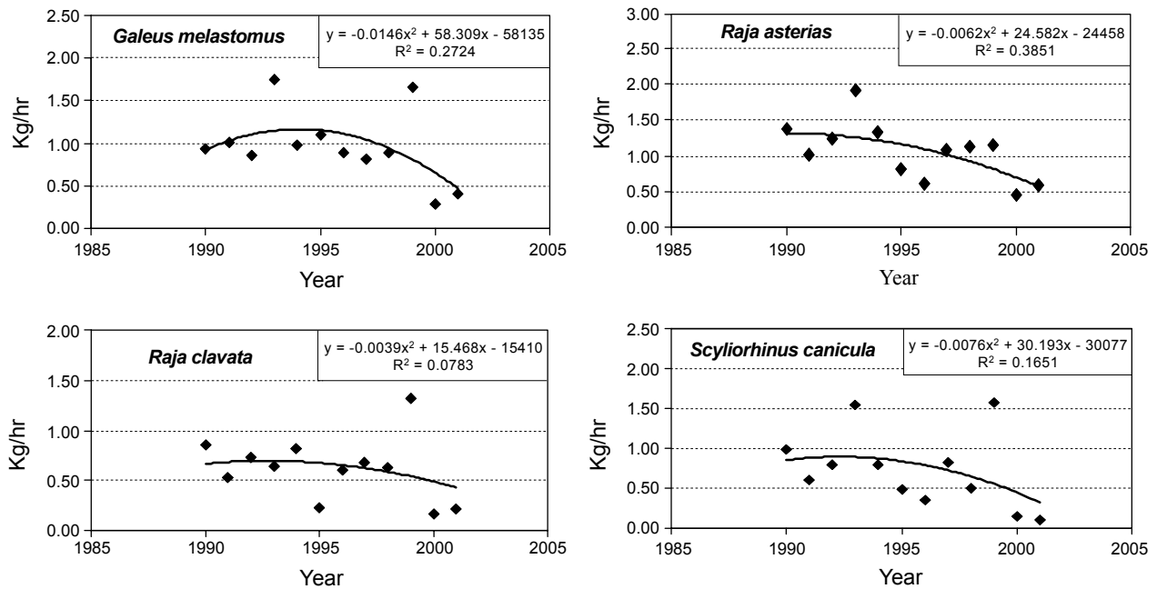
Fig. 5. Trends in catch rates (kg/hr) for G. melastomus , S. canicula , R. asterias and R. clavata for the commercial Viareggio fleet between 1990 and 2001.
