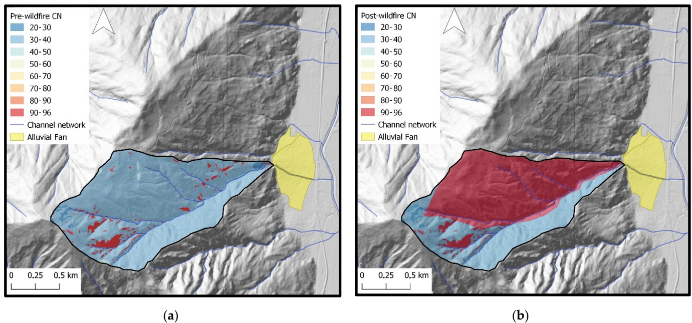
Figure 12. (a) Calculated CN for the Rio Casella catchment before the wildfire; (b) calculated CN for the Rio Casella catchment after the wildfire.
