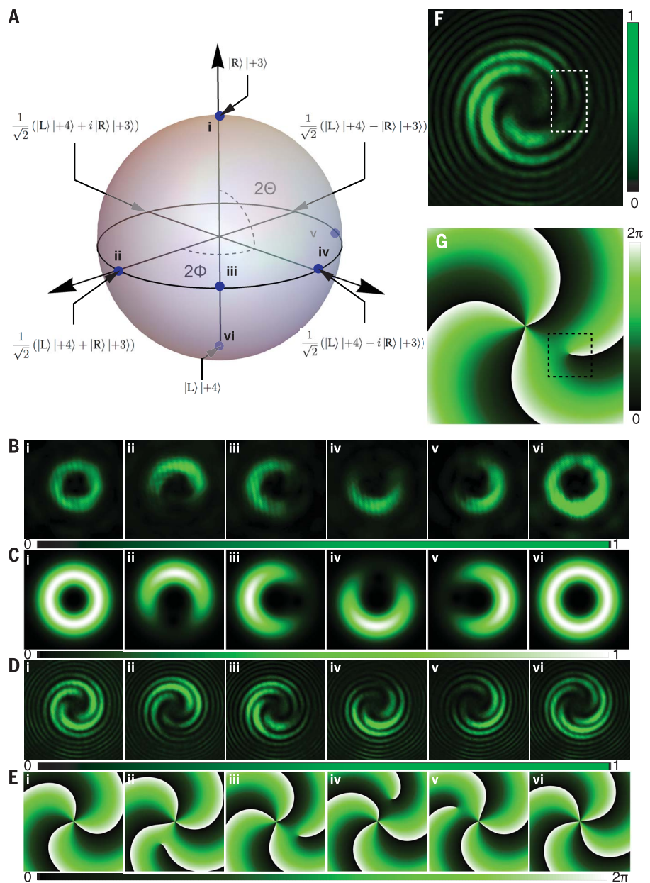
Fig. 2. Experimental demonstration of mapping from circular polarizations to two beams with arbitrary values of OAM.
