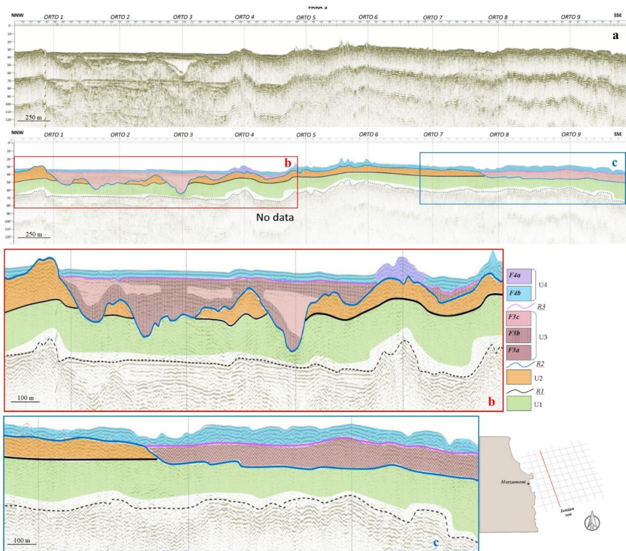
Figure 11. (a) Seismo-stratigraphic interpretation of the Para 3 profile, located in the central study area. (b) Seismo-stratigraphic interpretation of the northwestern and central portion of the Para 3 profile. (c) Seismo-stratigraphic interpretation of the southeastern portion of the Para 3 profile. Legend: refer to Figure 6.
