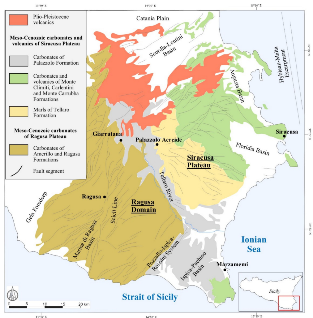
Figure 2. Schematic geological and structural map (WGS 84) of the Hyblean region (modified from [31]).
