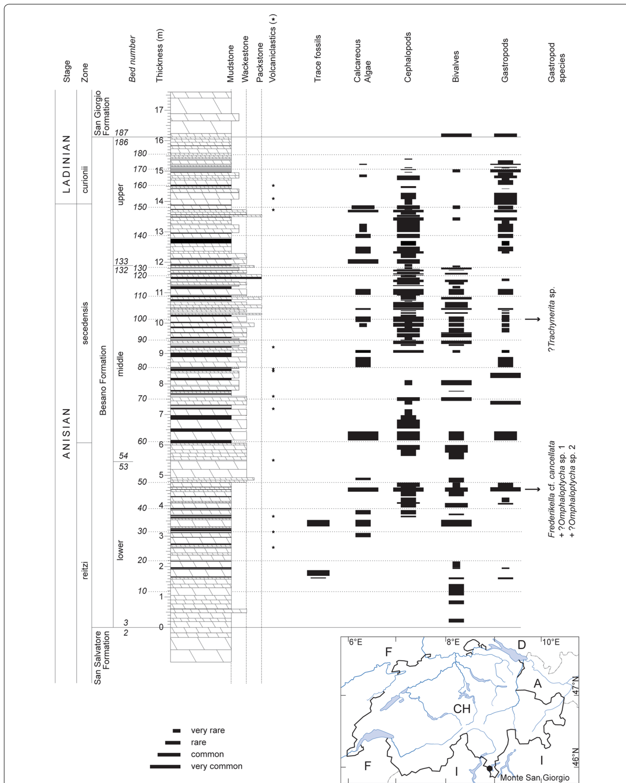
Fig. 1 Stratigraphic section of the Besano Formation at site Point 902/Mirigioli, with distribution and relative abundance of trace fossils, calcareous algae, cephalopods, bivalves and gastropods. Modified after Röhl et al. 2001 (Fig. 4), based on the internal inventory of the PIMUZ collection. The stratigraphic positions of four described specimens are indicated
