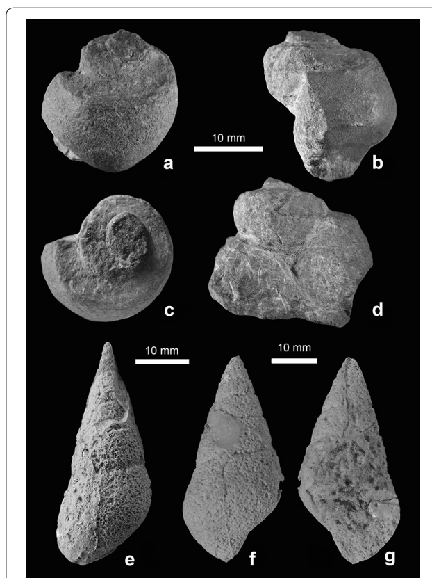
Fig. 4 a–d ? Trachynerita sp., Middle Besano Formation, uppermost Anisian. PIMUZ 37303: a apical side view, b side, c apical, and d abapertural view. e ? Omphaloptycha sp. 1, Lower Besano Formation, uppermost Anisian. PIMUZ 37312: Abapertural view. f, g ? Omphaloptycha sp. 2, Lower Besano Formation, uppermost Anisian. PIMUZ 29951: f abapertural and g apertural view. Images a–d have been obtained from original specimen; images e–g from silicon casts
