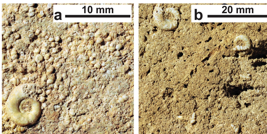
Fig. 5 Accumulations of small turriculate gastropods: larval-postlarval stages belonging to Caenogastropoda: a PIMUZ 37341 with a ceratitid ammonoid (lower left). Point 902/Mirigioli (Monte San Giorgio), Middle Besano Formation (bed 76); b PIMUZ 37340, three silicified gastropods (bottom and upper right) together with two silicified ceratitid ammonoids ( Reposia acutenodosa Rieber, 1973). Valle Stelle (Monte San Giorgio), Middle Besano Formation (bed 69)
