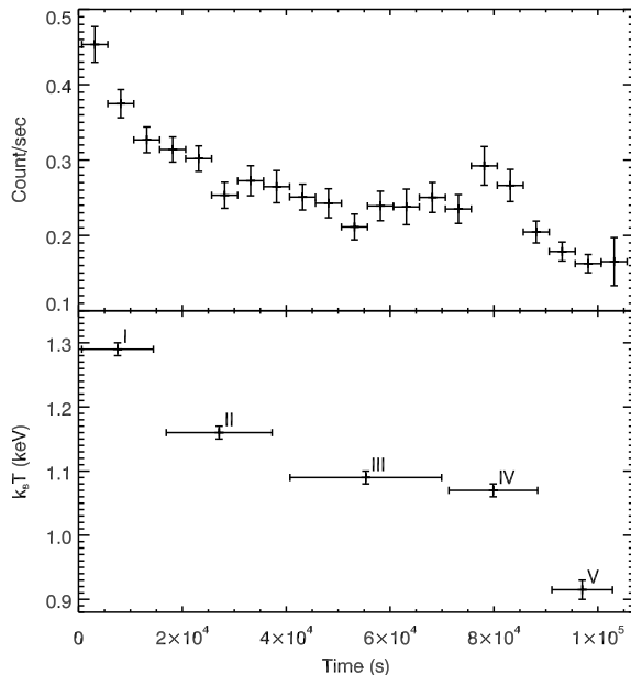
Figure 4. Background subtracted MECS 2–10 keV light curve and blackbody temperature observed on 2001 April 18 about 7.5 hours after the flare. See Table 4 for the latter values, obtained from the addition of a new blackbody component with fixed emitting area. The time intervals with bursts have been excluded. Error bars are at 1\sigma .
