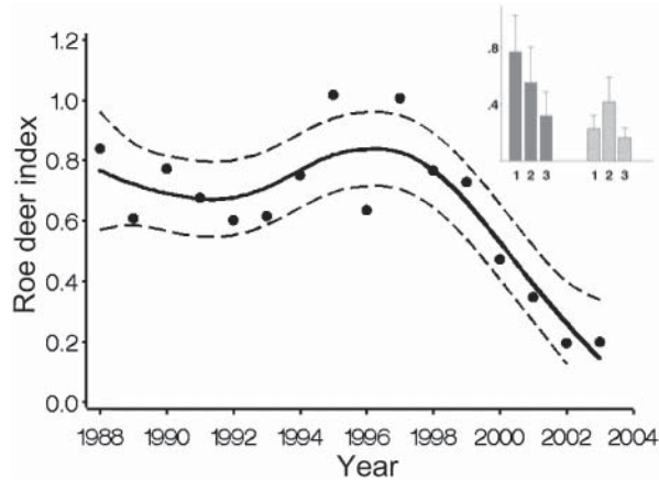
Fig. 2 Variations in the roe deer index from 1988 to 2003, with generalized additive modelling regression (solid line) and 95% confidence limits (dashed lines). In the inset, the index is given separately for Capocotta (dark grey) and Castelporziano (light grey) in 2001, 2002 and 2003 (denoted 1, 2 and 3, respectively) with the corresponding 95% confidence limit (thin vertical bar).
