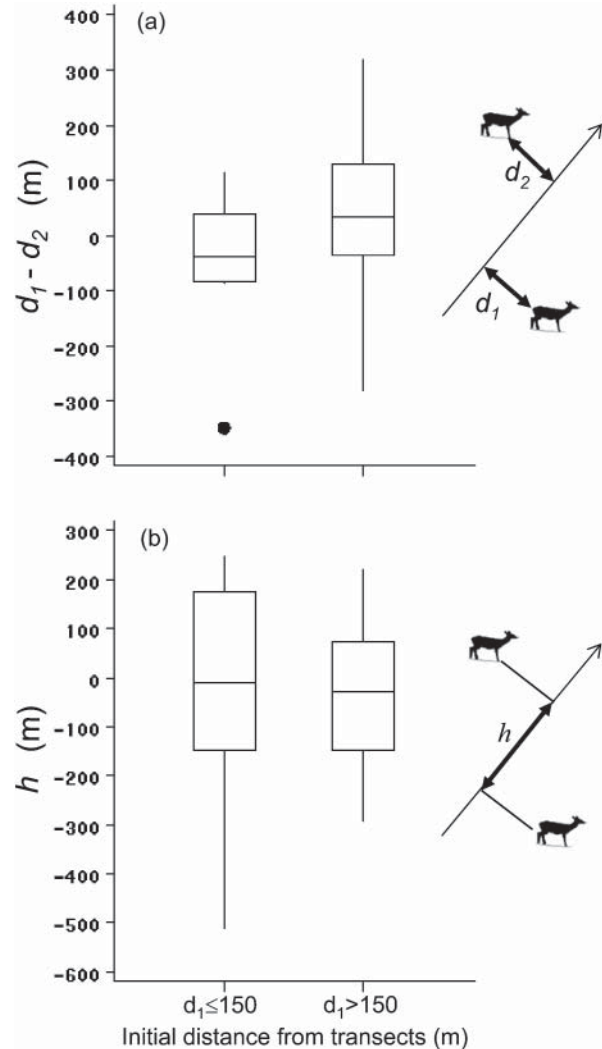
Fig. 5 Box-and-whisker plots of (a) the difference between the perpendicular distances of roe deer from the transect line before ( d_1 ) and after ( d_2 ) a transect was walked, and (b) the difference ( h ) between the projections of the locations of roe deer onto the transect line before and after a transect was walked, for deer 'near' ( d_1 \leq 150 m) and 'far' ( d_1 > 150 m) from the transect. Negative values of ( d_1 - d_2 ) indicate that the animal moved away from the transect and negative values of h indicate that animals moved away from the observer.
