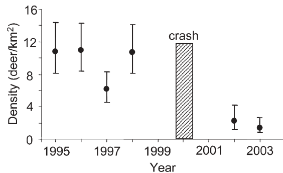
Fig. 4 Estimates of roe deer density for 1995–2003, using distance sampling. From 1995 to 1998 data were collected only at Castelporziano, but at both Castelporziano and Capocotta in 2002–2003.
