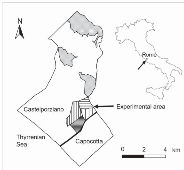
Fig. 1 The study areas of Castelporziano and Capocotta. Fenced areas used for agriculture are in grey. The shading patterns distinguish the four counting zones of the experimental area (see text for details).
