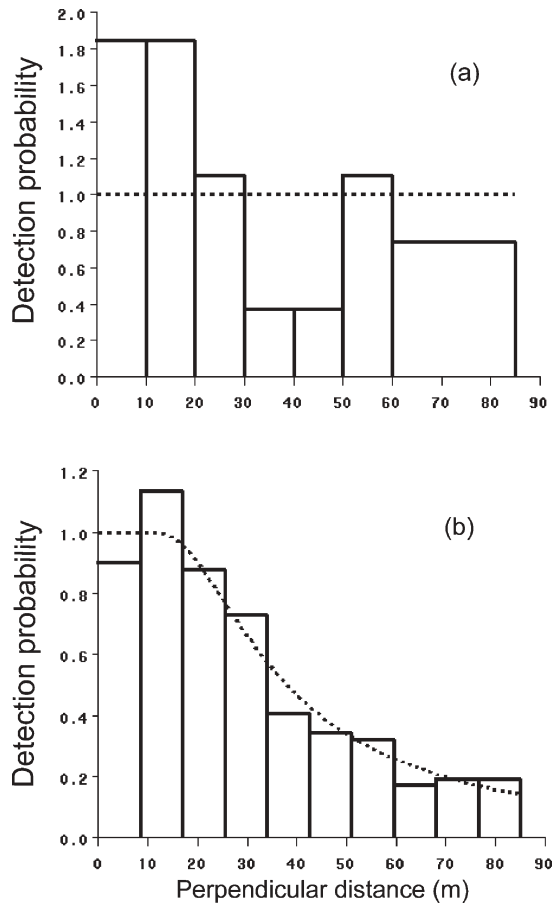
Fig. 3 Histogram of the detection probability of roe deer at increasing perpendicular distances from the transect centre line, and the detection function (dotted line) for (a) the experimental survey in spring 2003 (uniform key) and (b) of the selected model 1 (Table 1; hazard rate key).
