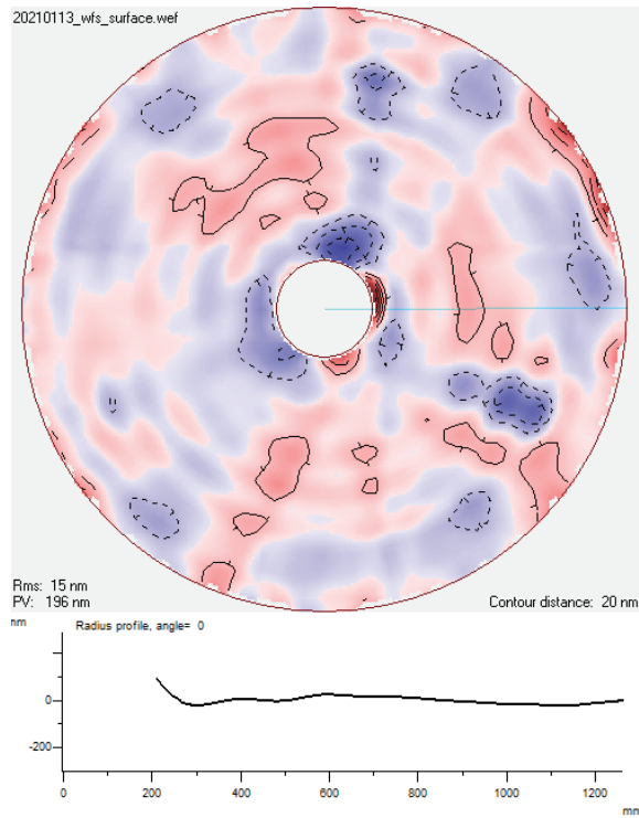
Figure 7. Latest surface accuracy measurement performed at OPTEON.
