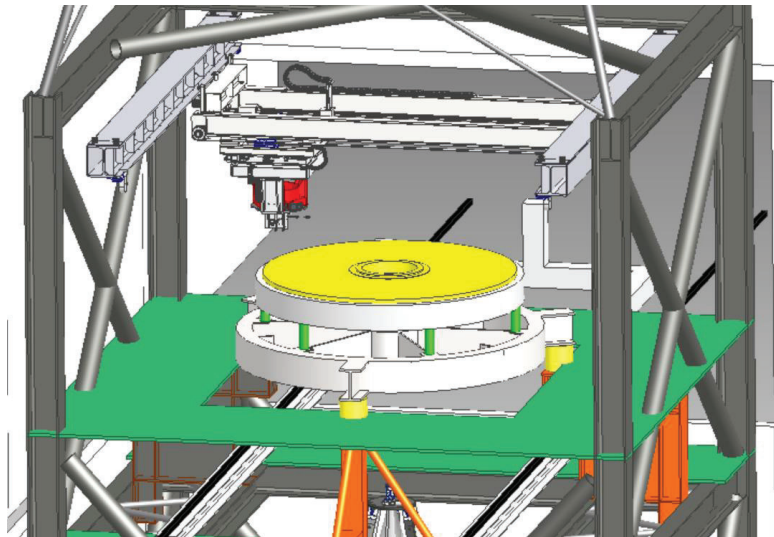
Figure 9. ATHENA MAM structure and Handling and Alignment Device
