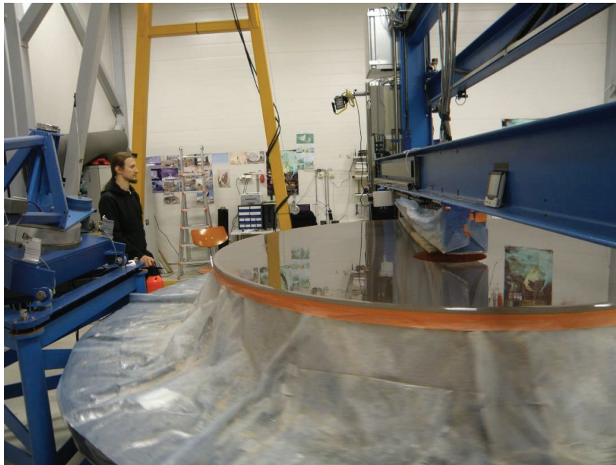
Figure 6. Polishing of the 2.6 m UV collimator at OPTEON Oy.
