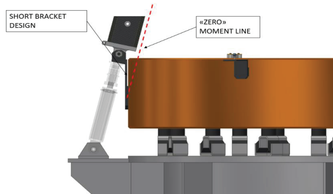
Figure 5. Gravity release mechanism for the 3 legs of the CFRP structure.
