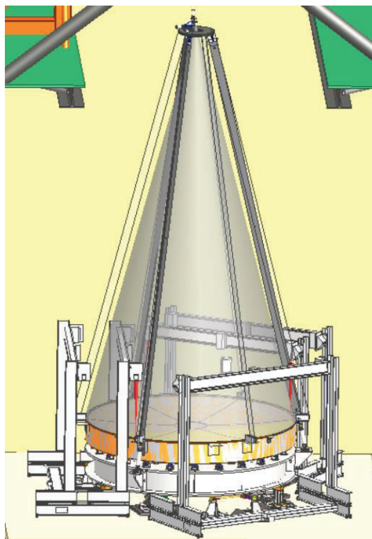
Figure 4. UV source supporting structure (above the mirror) and the 54 pads below the mirror.
