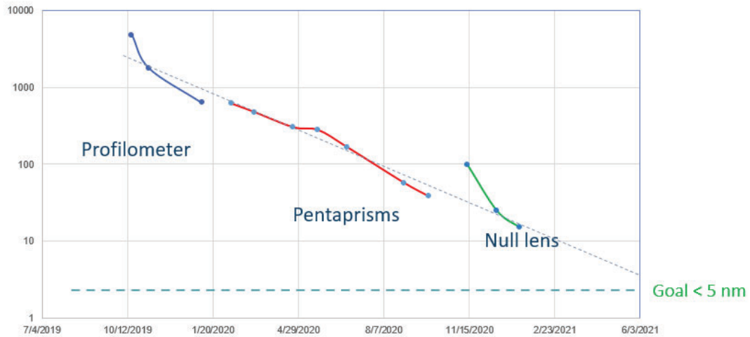
Figure 8. Surface accuracy of the Collimator mirror versus time
