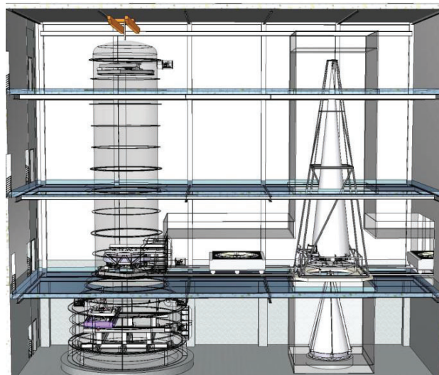
Figure 3. ATHENA building with VERT X (left) and ATHENA AIT (right)
