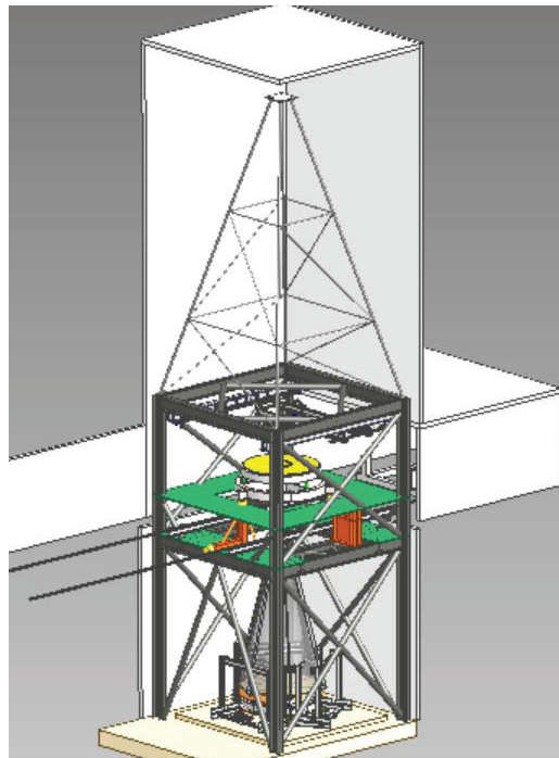
Figure 1. UVOB Cross section.
