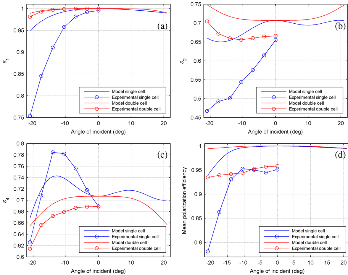
Fig. 13 Comparison between experimental and theoretical polarimetric efficiencies of the PMPs with single- and double-cell configuration as a function of the AOI. (a) \epsilon_1 , (b) \epsilon_2 , (c) \epsilon_4 , and (d) \epsilon_{total} .
