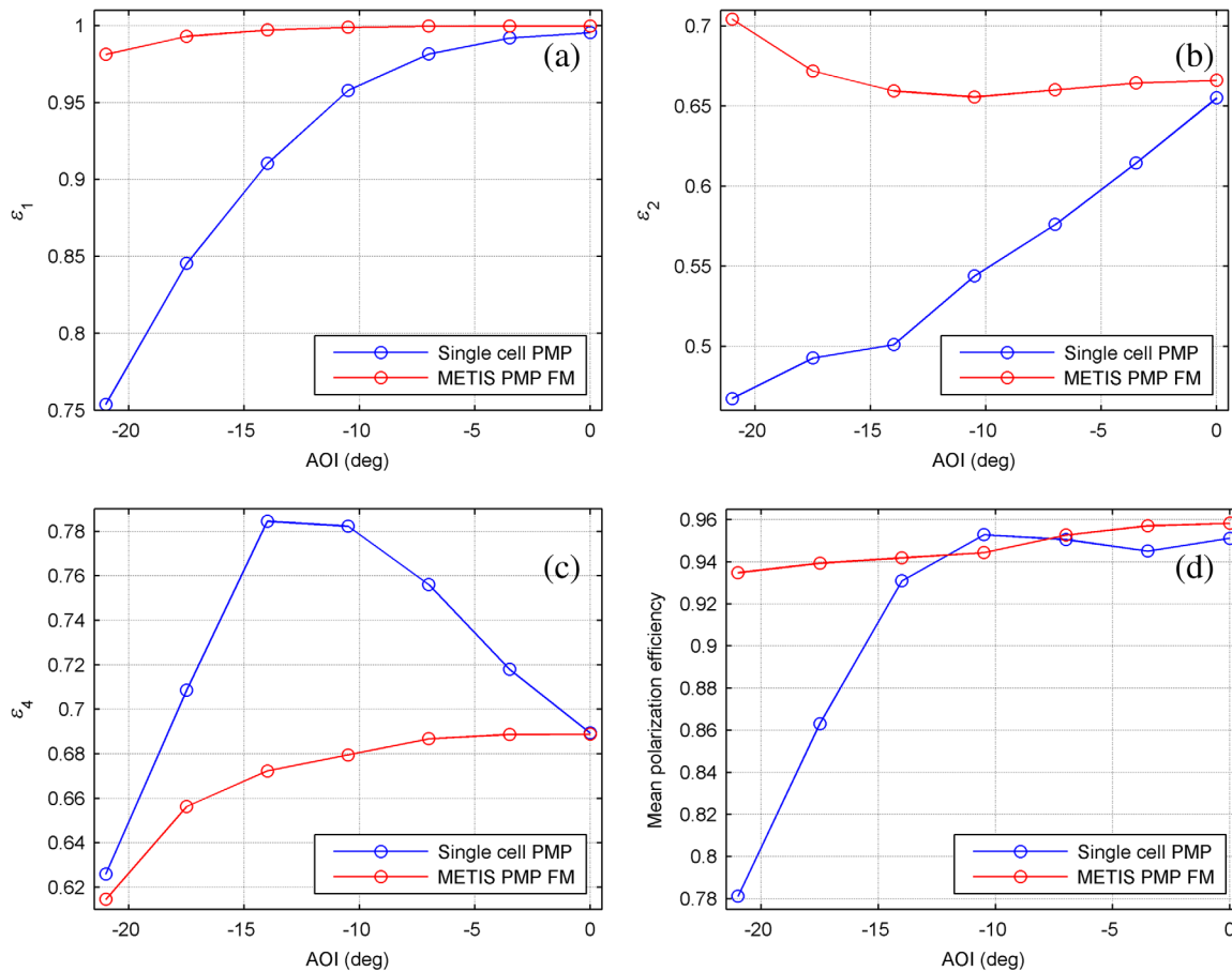
Fig. 11 Modulation efficiencies measured experimentally at a different AOI for PMP with single- and double-cell configuration. (a) \epsilon_1 , (b) \epsilon_2 , (c) \epsilon_4 , and (d) \epsilon_{total} .
