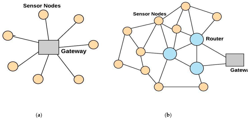
Figure 3. (a) Star topology, (b) mesh network topology.
