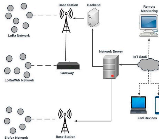
Figure 6. Internet of Things (IoT) mixed architecture.
