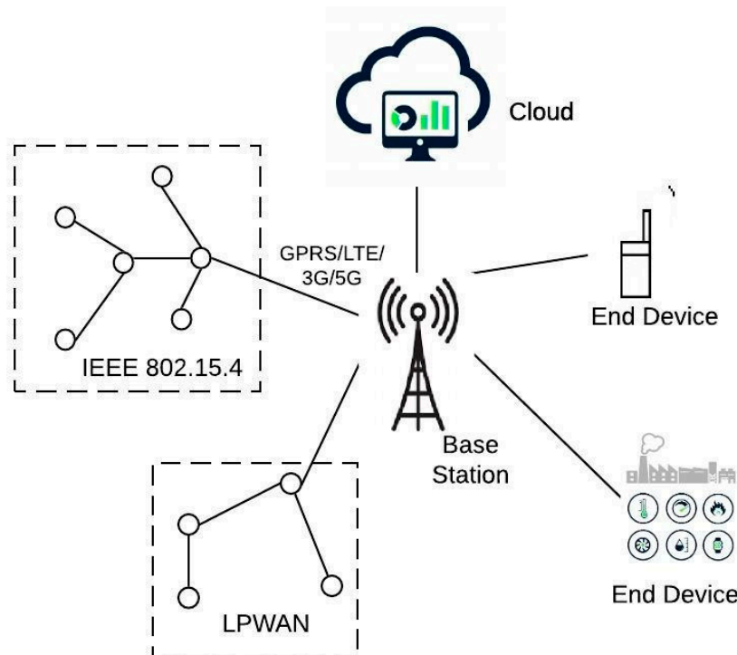
Figure 5. Generalized cellular type architecture.
