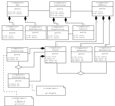
Fig. 2. The class diagram of the overall control system
