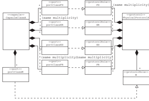
Fig. 1. UML-RT representation of a physical subsystem
