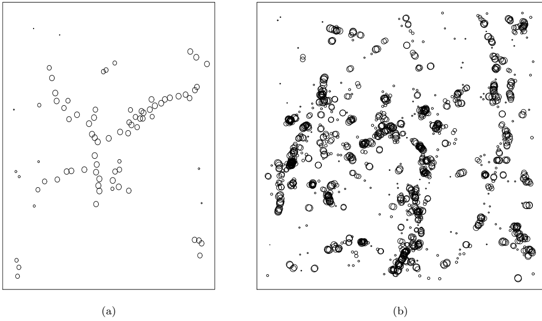
Figure 9: Scatter plot with circles indicating the marginal posterior probability of a point being a cluster point for (a) the mountain tops data set and (b) the barrows data set.
