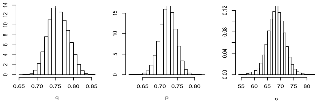
Figure 6: Histograms showing the marginal posterior distributions of q , p , and \sigma for the barrows data set.
