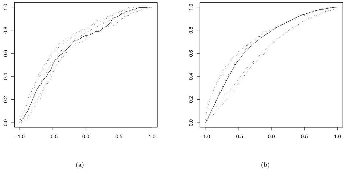
Figure 12: (a): The distribution function for squeezedness q_{i,j} for the mountain tops data set (solid line) and 0.5 %, 2.5 %, 50 %, 97.5 %, and 99.5 % quantiles obtained from 199 posterior predictions. (b): A similar plot for the barrows data set.
