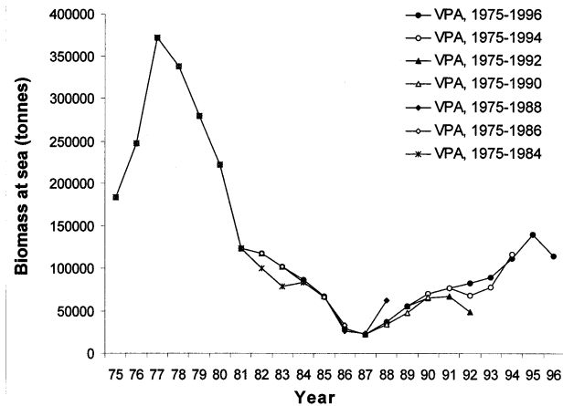
FIG. 6. - Mid-year anchovy biomass at sea estimated by retrospective VPA, using data for different time intervals, from 1975 to 1996/94/92/90/88/86/84. These VPAs were carried out using the fishing mortality rate F_{3,1996} = 0.5 and natural mortality rate M = 0.6 . Calendar year data were used.
