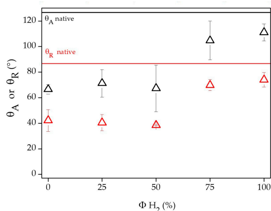
Figure 5. Variation of advancing and receding WCAs of PCL scaffolds treated with Ar, Ar/H 2 , or H 2 as a function of the feed composition: black triangles represent \theta_A ; red triangles represent \theta_R ; black continuous line represents \theta_A for native scaffold ( 129 \pm 3^\circ ); red continuous line represents \theta_R for native scaffold ( 88 \pm 1^\circ ).
