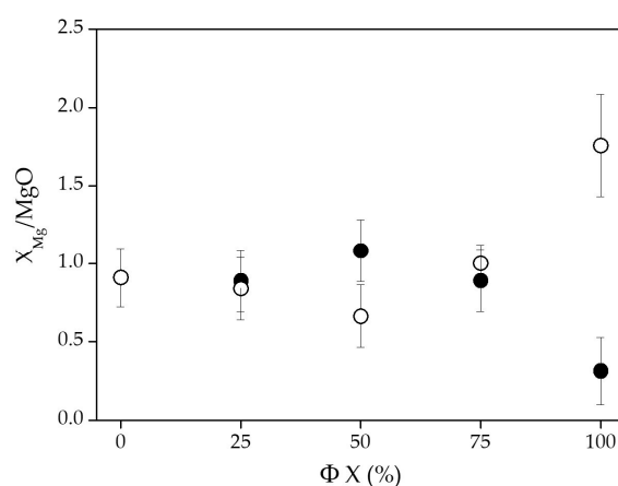
Figure 3. Variation of the X Mg /MgO ratio resulting from the curve-fitting of the XPS high-resolution Mg2p spectra as a function of the gas feed composition for plasma-processed PCL flat samples. Note: • = H 2 O; o = H 2 .
