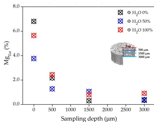
Figure 4. XPS surface magnesium percentage ( Mg_{Tot} %) in the core of PCL scaffolds as a function of the sampling depth from the top.
