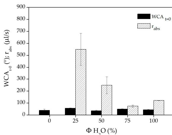
Figure 6. Water absorption rate and WCA values at absorption time zero for PCL scaffolds treated with Ar, Ar/H 2 O, or H 2 O feed as a function of the feed composition.
