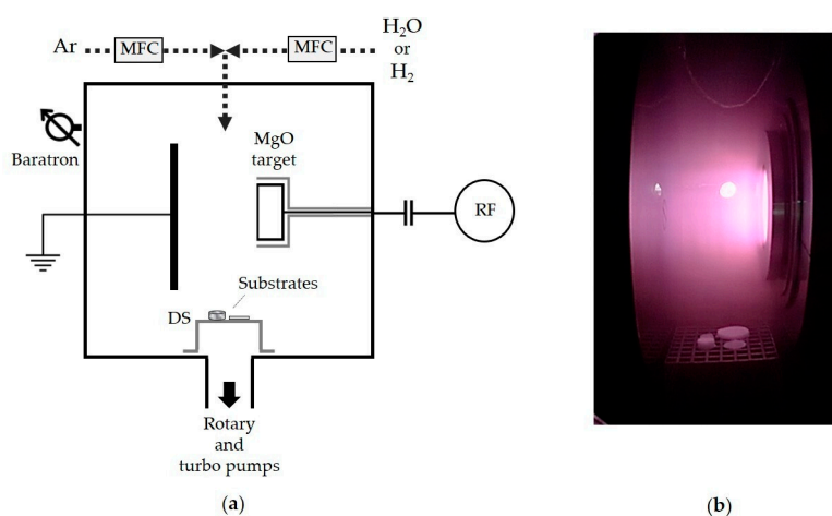
Figure 1. (a) Schematic representation of the asymmetric plasma reactor; (b) Photograph of discharge during a deposition process.
