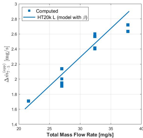
Figure 13. Apparent variation of ingested mass flow rate, indicated as \Delta\dot{m}^{(app)}_{7-5} calculated from the thrust variations and comparison with the background flow model (with an amplification factor \beta = 49.6 ) for HT20k L.
