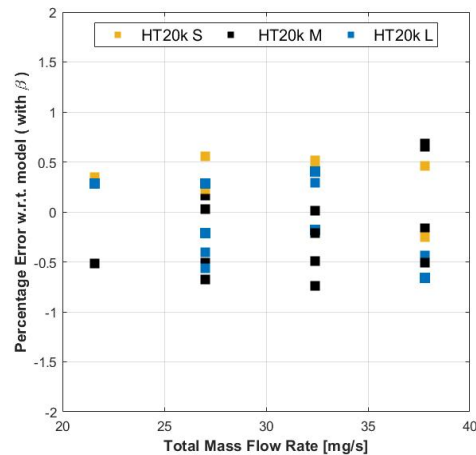
Figure 14. Percentage error regarding the model (with \beta = 49.6 ) for all 3 configurations; the \Delta\dot{m}^{(app)}_{7-5} was calculated from thrust variations.
