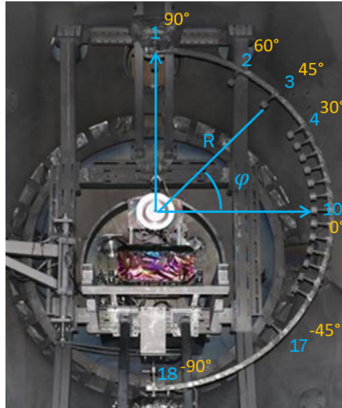
Figure 4. Faraday probes arrangement—the thruster is the HT5k [25].
