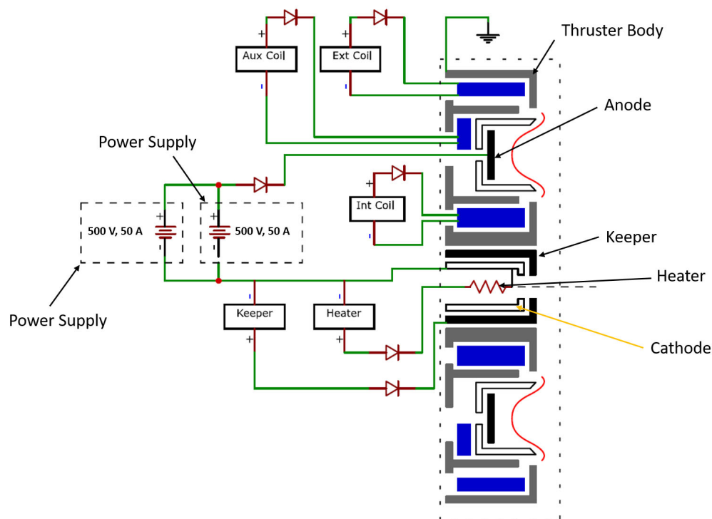
Figure 3. Electrical scheme—the thruster body was grounded.
