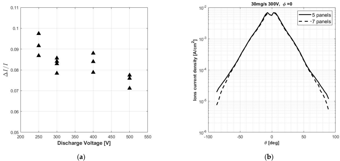
Figure 11. Variations of the discharge current as a function of the discharge voltage for the HT20k M configuration (a). Beam current density distribution for the for the Faraday probe at \phi = 0^\circ for \dot{m}_a = 30 mg/s and V_d = 300 V with 5 and 7 cold panels (b).
