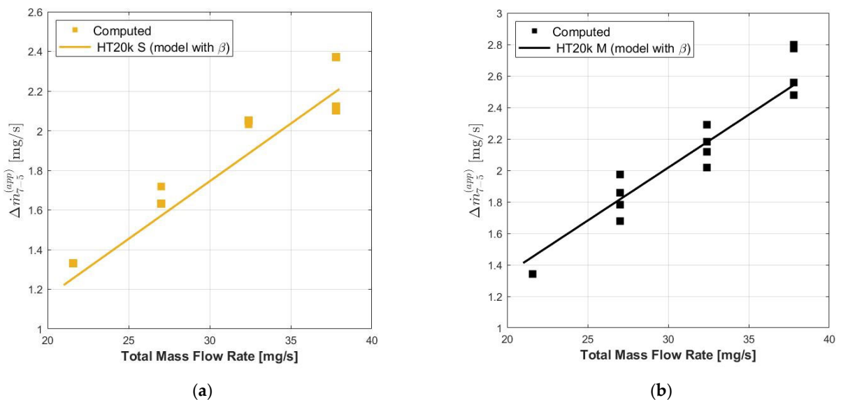
Figure 12. Apparent variation of ingested mass flow rate, indicated as \Delta \dot{m}^{(app)}_{7-5} calculated for the thrust variations and comparison with the background flow model (with an amplification factor \beta = 49.6 ) for HT20k S (a) and HT20k M (b).
