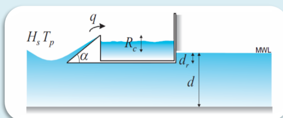
Fig. 3 – Sketch of the 2D setup used in the tests
