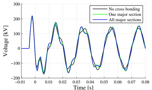
Figure 15. Measured and simulated phase to ground voltage at the sending end using all major sections, one major section, and no cross-bonding.
