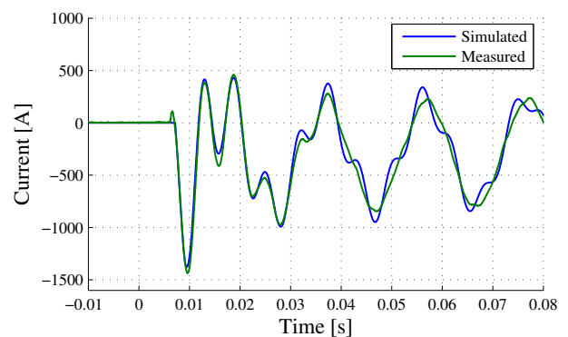
Figure 12. Simulated and measured high resolution current flowing in phase b measured at station Endrup.
