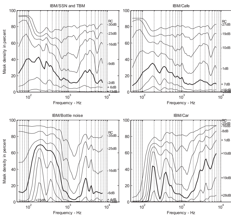
FIG. 5. Mask density (in percentage of mask value 1) as function of channel center frequency averaged over entire sentence material. The corresponding RC value used for computing the mask is indicated to the right of each curve. The bold line corresponds to the RC value with the highest intelligibility for IBM-gated noise (at mixture SNR of -60 dB). The mask densities of the TBM masks equals that of the IBM/SSN by definition.
