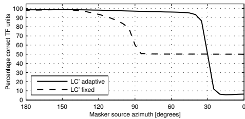
Fig. 4. The percentage of correct T-F units in the \widehat{IBM} with respect to the IBM. The target was fixed at 30^\circ while the masker was moved from 180^\circ to 0^\circ . The adaptive LC' value was calculated from the directional gains using an LC value of 0 dB, whereas the fixed LC' was kept at 0 dB.
